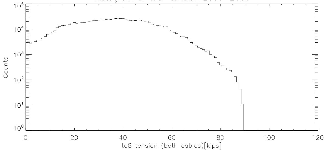
Histogram of td8 tension 2008-2009
