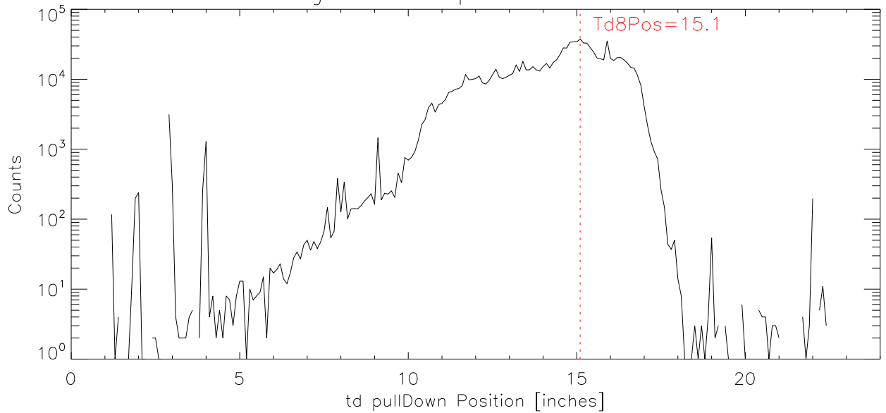
Histogram of td8 position 2008–2009
