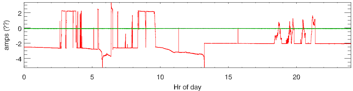
drive current (from amp monitor)
