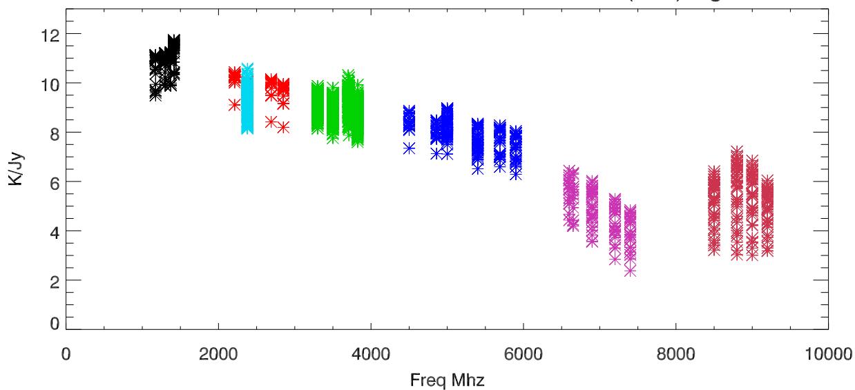
mar11-mar12 Gain lband to xband rcvrs. za=(5-14)deg
