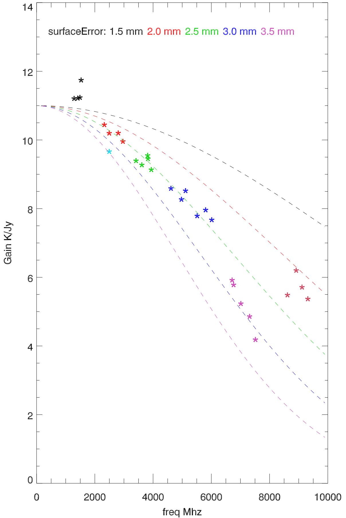
mar11-mar12 median gain vs freq. With ruzeCurves. za-(5-14)
