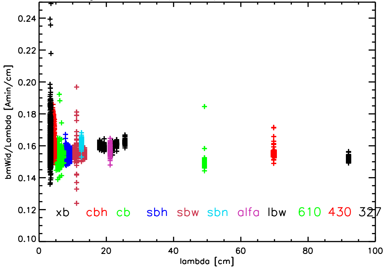
(average_Beam_Width/lambda) vs lambda (2004-2005)
