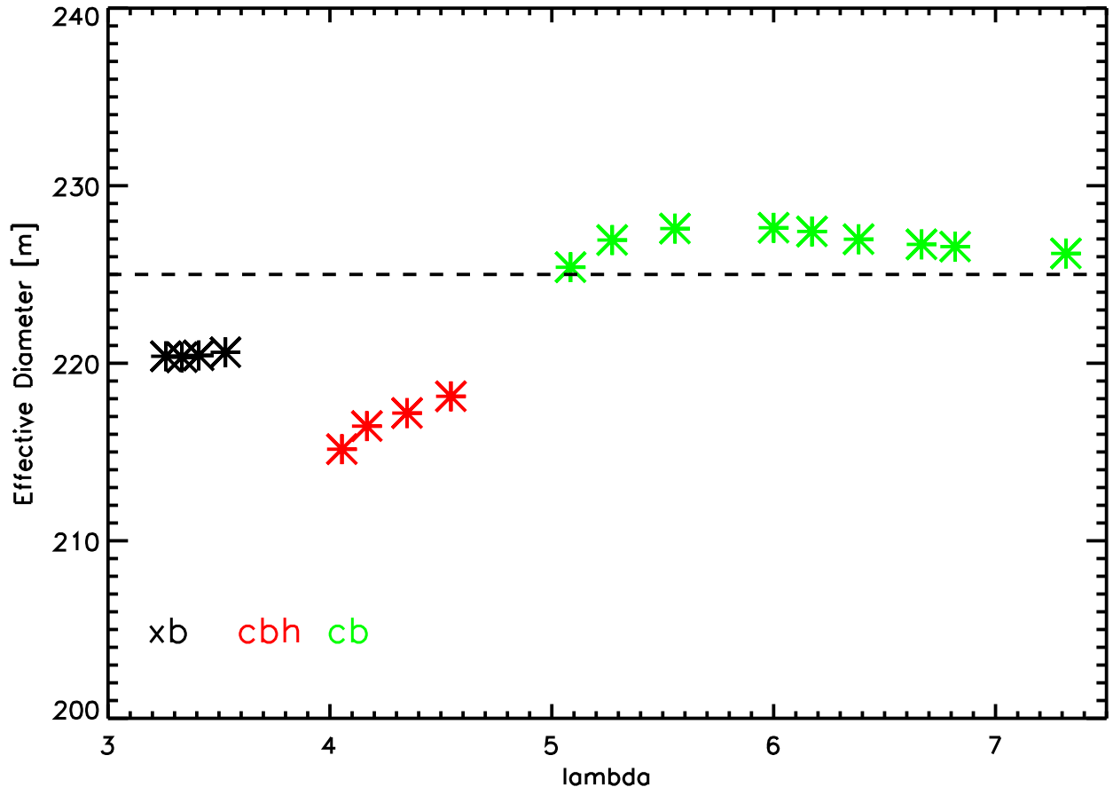
Effective Diameter dish vs lambda
