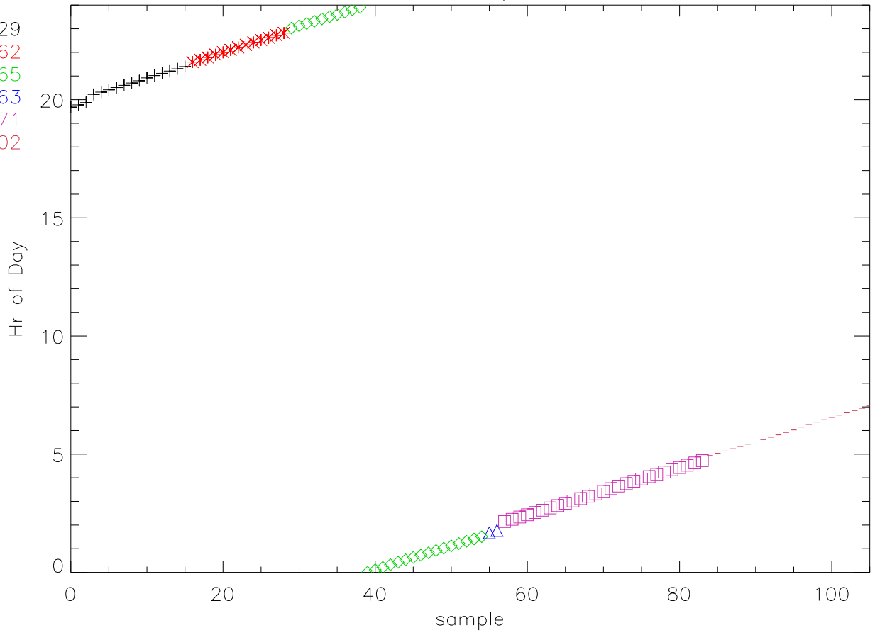
alfa hour of day for data
