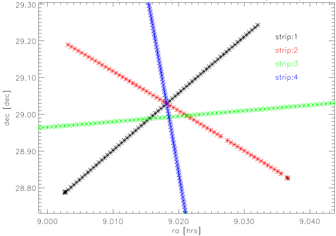
01nov04 spider scan positions after fix (beam0)
