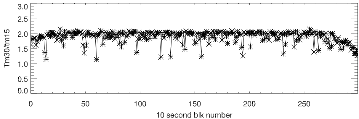
FFT time Ratio: Time30threads/Time15Threads
