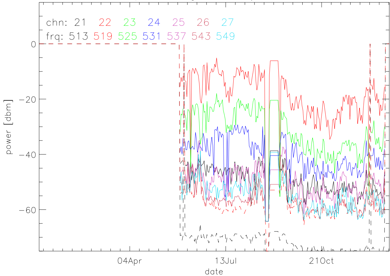
TV stations hilltopMonitoring 2004:daily min. 550Mhz RfiBand
