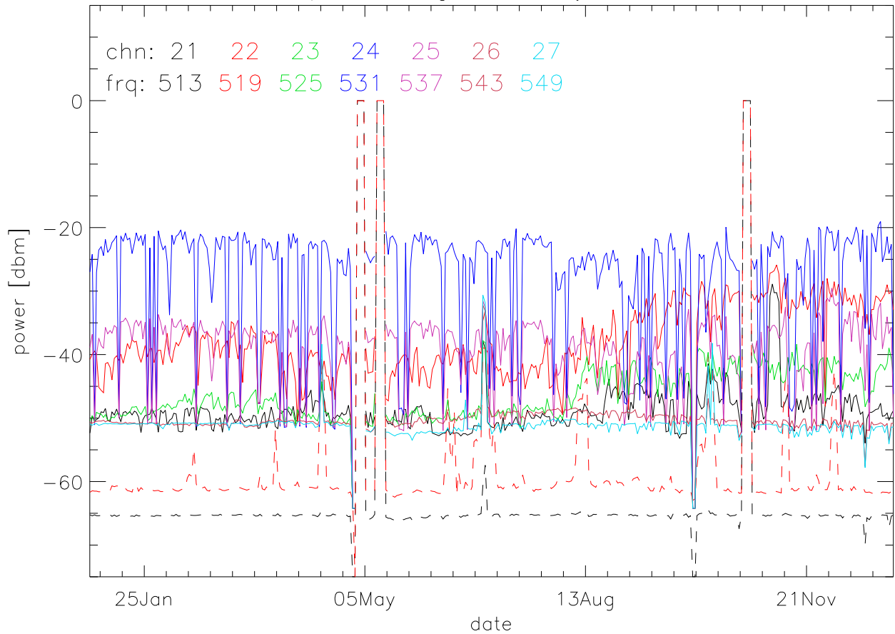
TV stations hilltopMonitoring 2002:daily min. 550Mhz RfiBand
