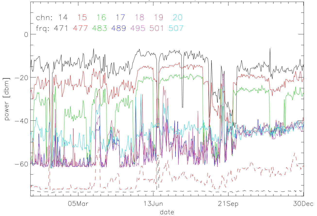
TV stations hilltopMonitoring 2006:daily max. 550Mhz RfiBand
