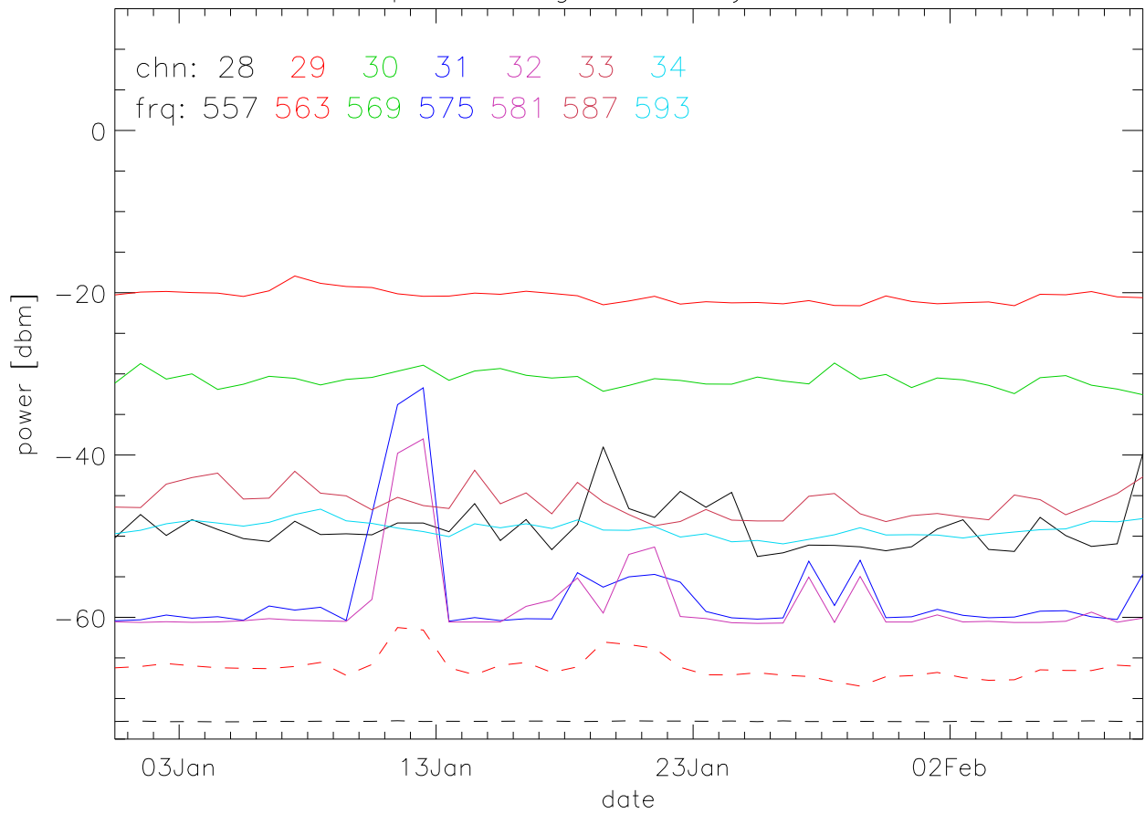
TV stations hilltopMonitoring 2012:daily max. 550Mhz RfiBand
