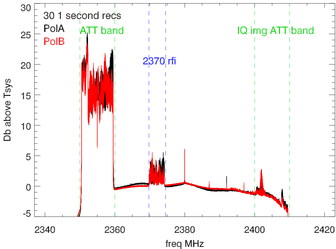
15aug17 sbn. spectra showing 2370 rfi
