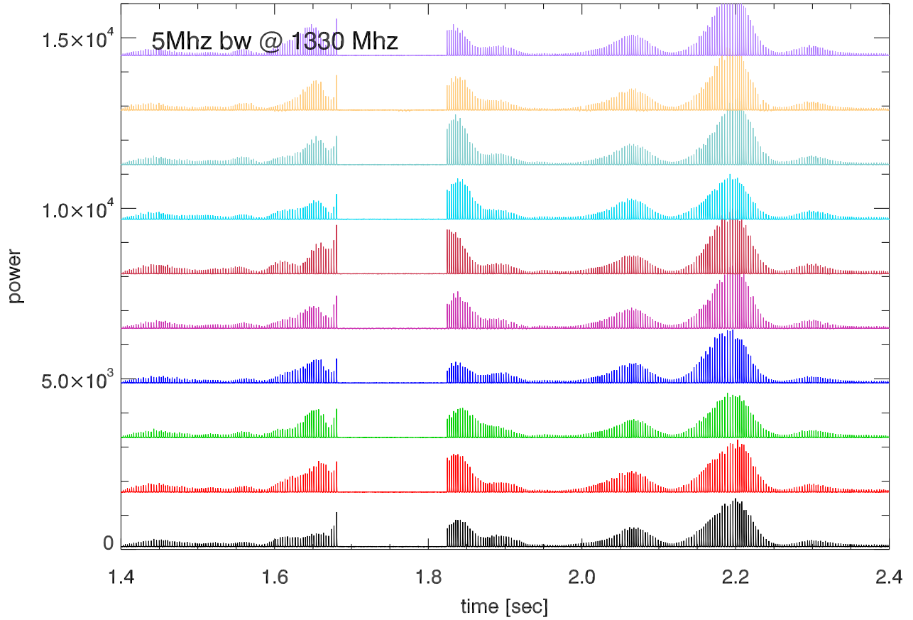
04oct13 PuntaBoringquenRdrl totalPwr vs time for 10 rotations
