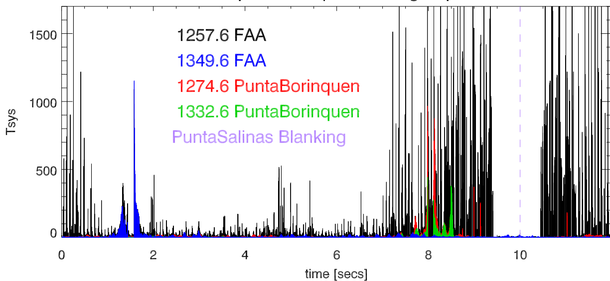
01nov11 faa,puntaBorinquen blanking. totpwr vs time
