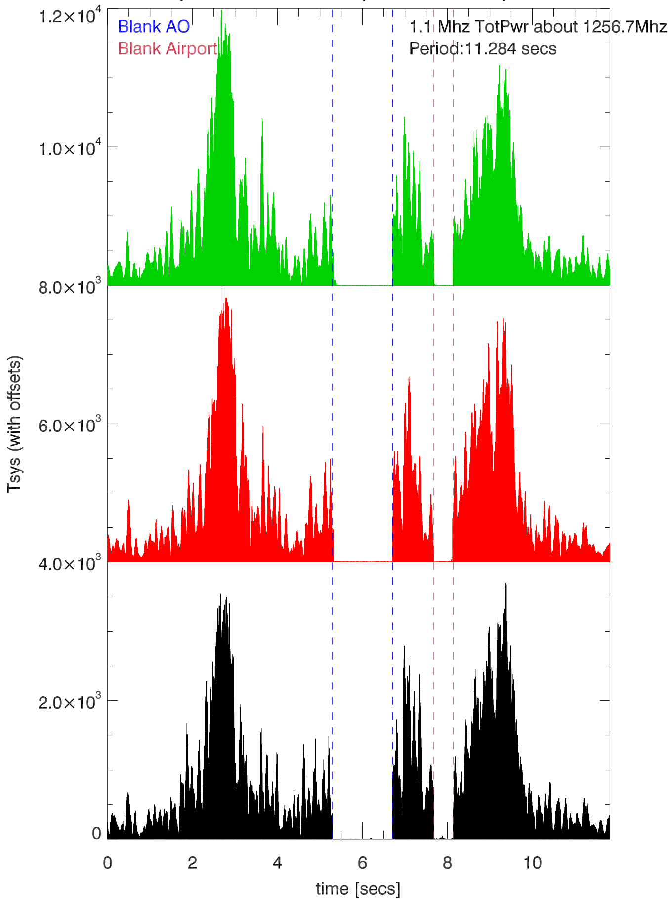
22apr14 Aerostat total pwr vs time. 3 periods
