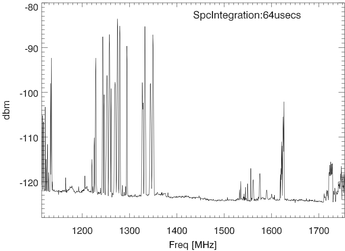
Peak hold spectra
