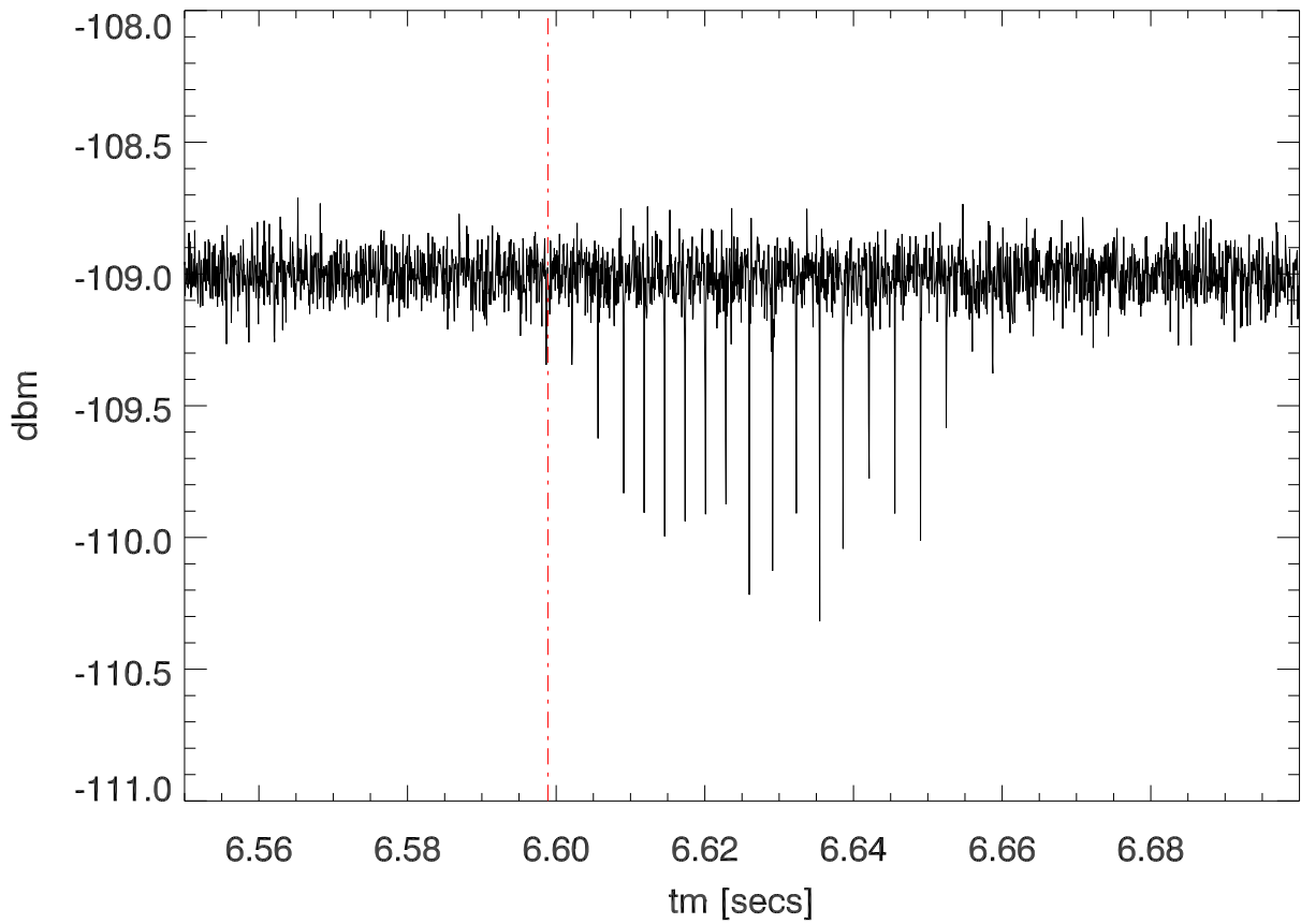
lbw 1390-1420 total pwr vs time (blowup)
