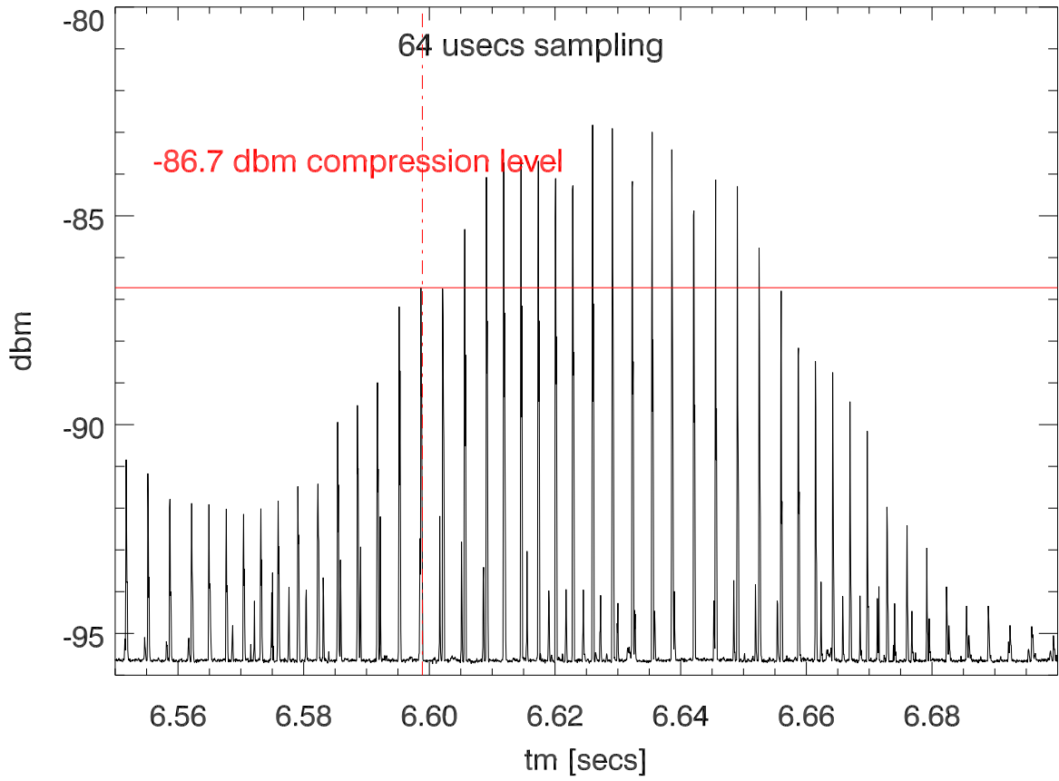
190305: lbw totPwr vs time (blowup around saturation)
