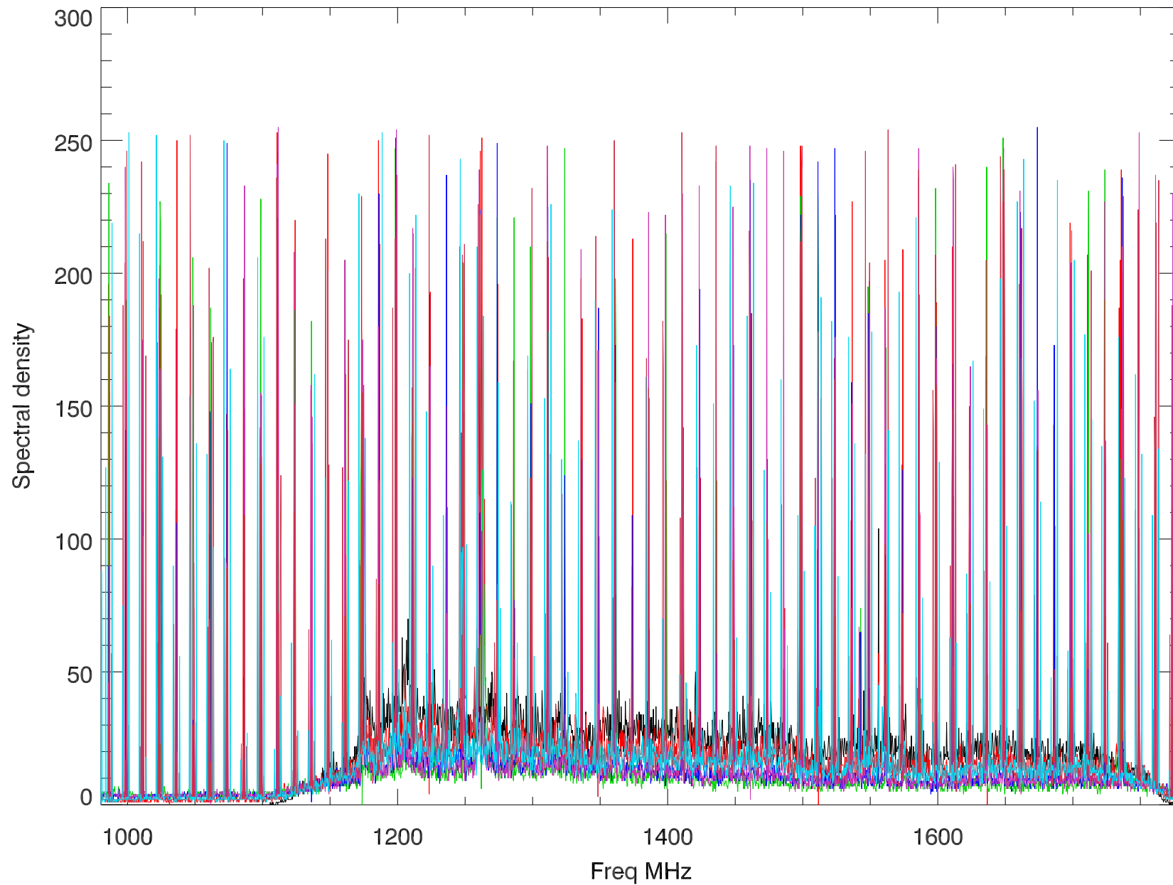
P2789 overplot 7 40usec spectra during 78.9725 sec compression
