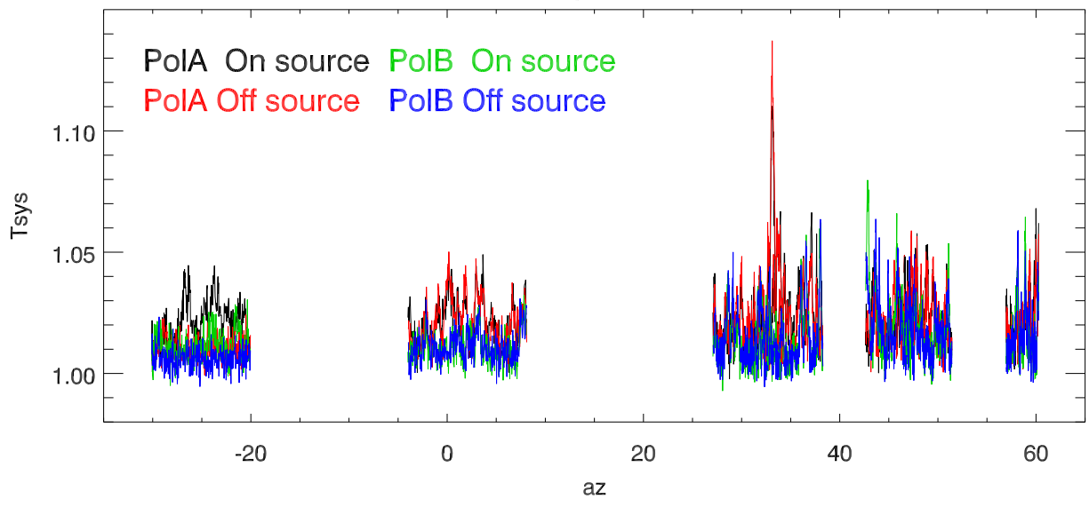
a2335: 14mar11 1357.3 rfi tp vs azimuth: 1357.3/baseline)
