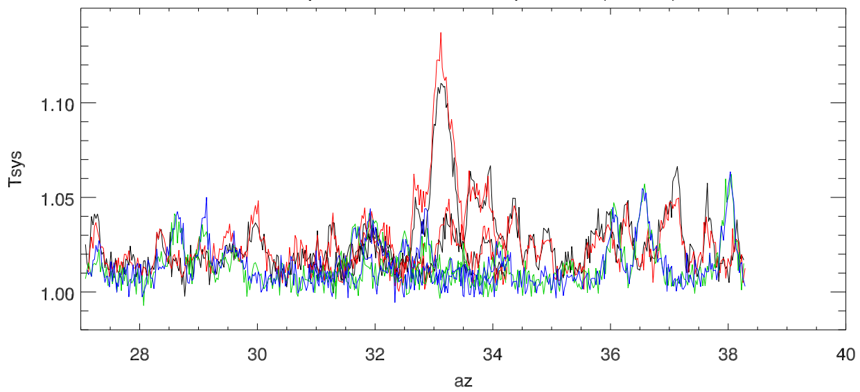
blowup around distomat 1 position (az=35)
