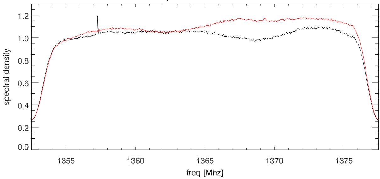
Spectrum for rfi max
