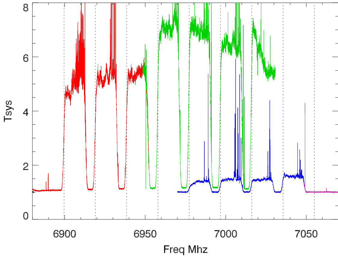
peak rfi spectra 11mar13 and 16mar13
