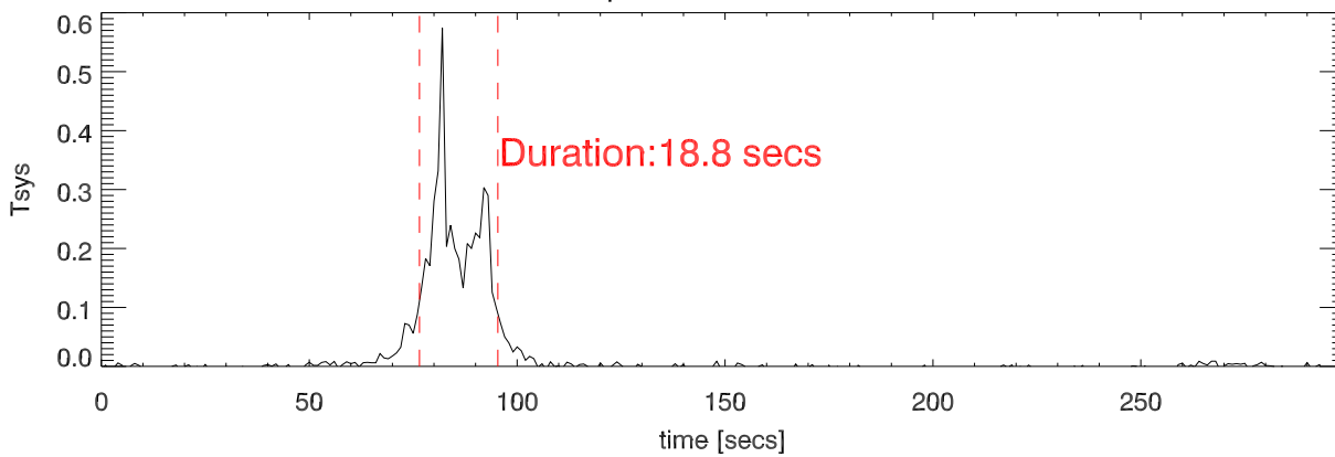
16mar13 total power 7020-7025 Mhz vs Time
