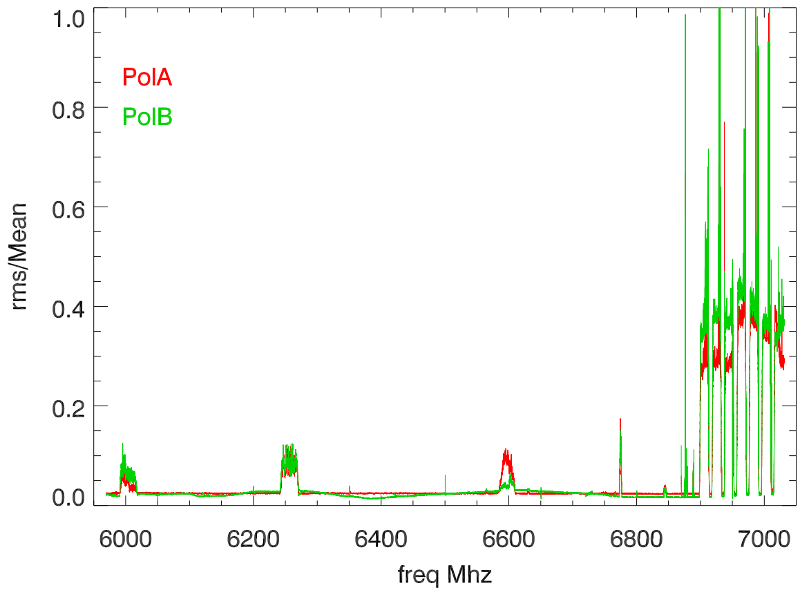
11mar13 a2675 file 1900 all bands. rms/mean for 300 recs
