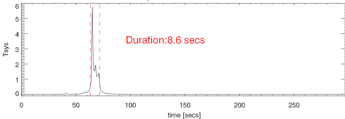
11mar13 total power 6980.5-6985.5 Mhz vs Time
