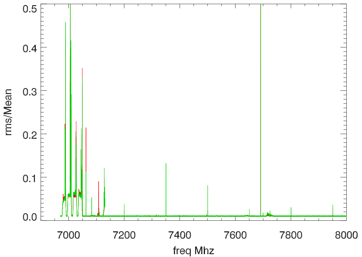
16mar13 a2675 file 2200 all bands. rms/mean for 300 recs
