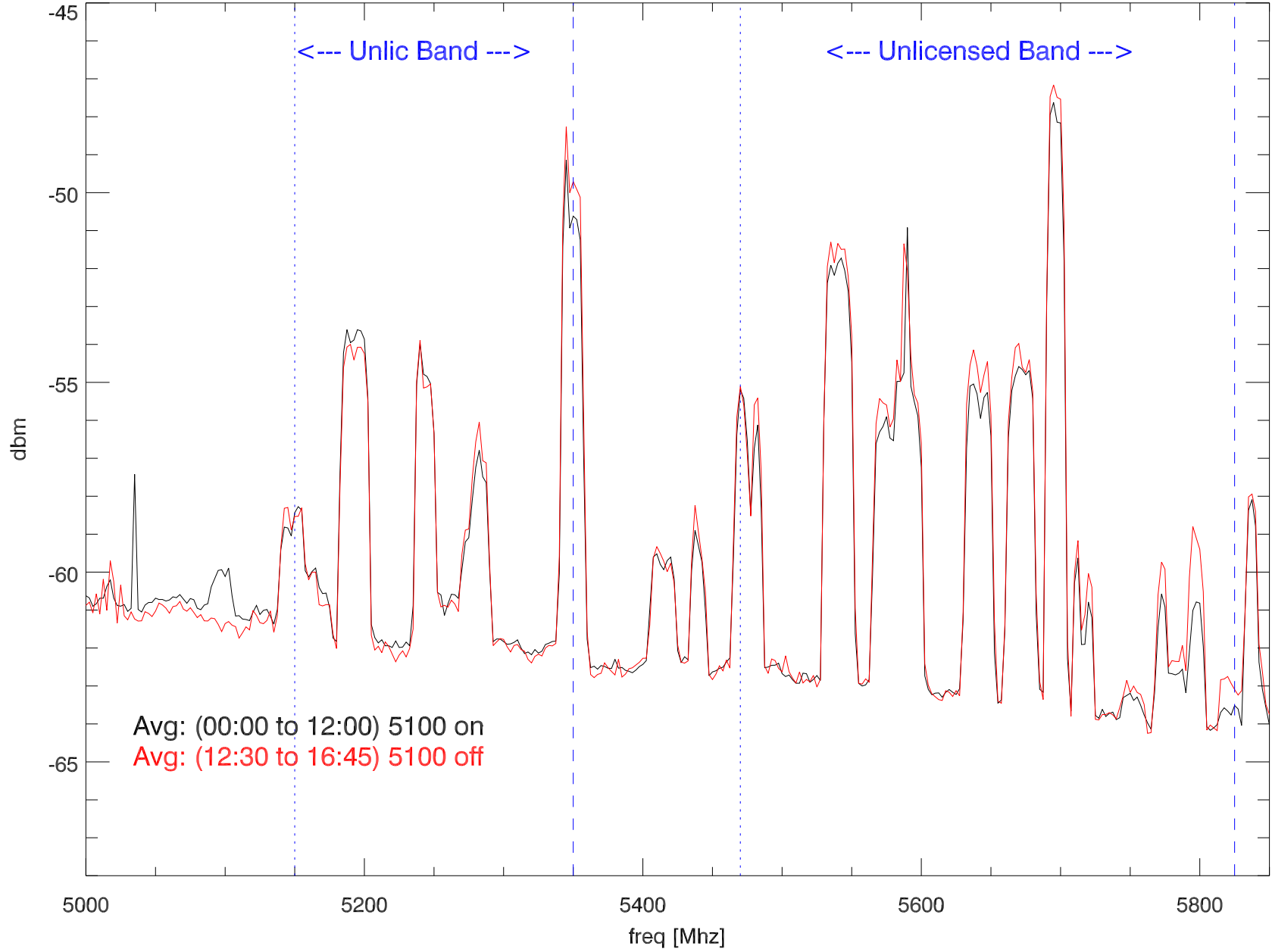
05jun13 hilltop avgSpectra showing 5100 turnoff
