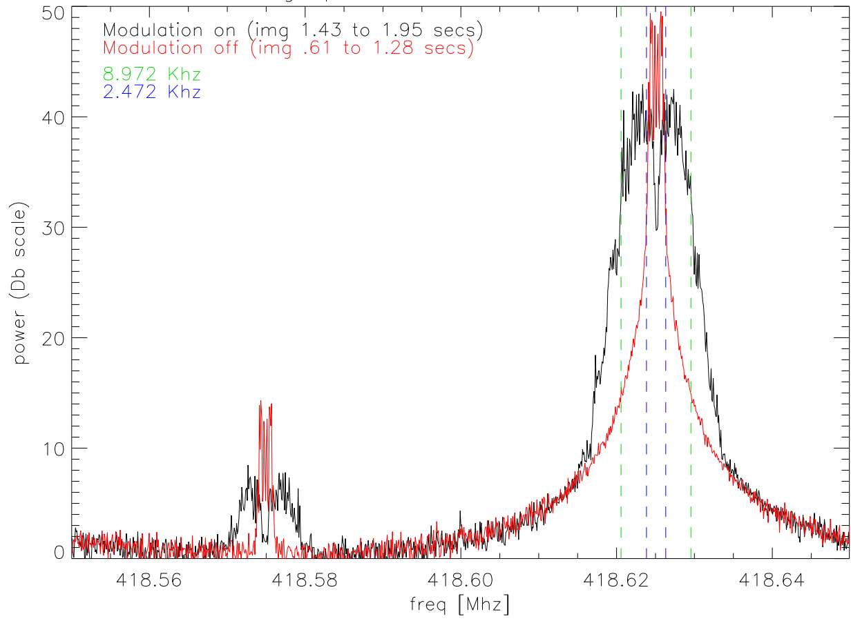
01dec06 Avg Spectra modulation on, modulation off
