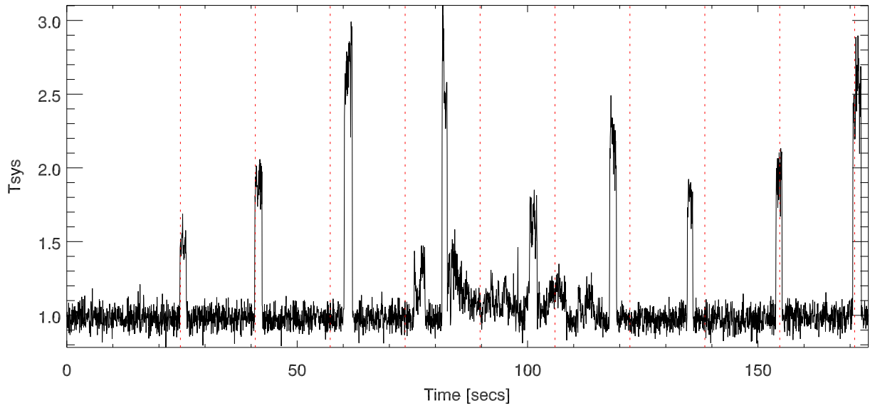
30nov12 430gr periodic rfi. Freq:434.68 Period: 10.00
