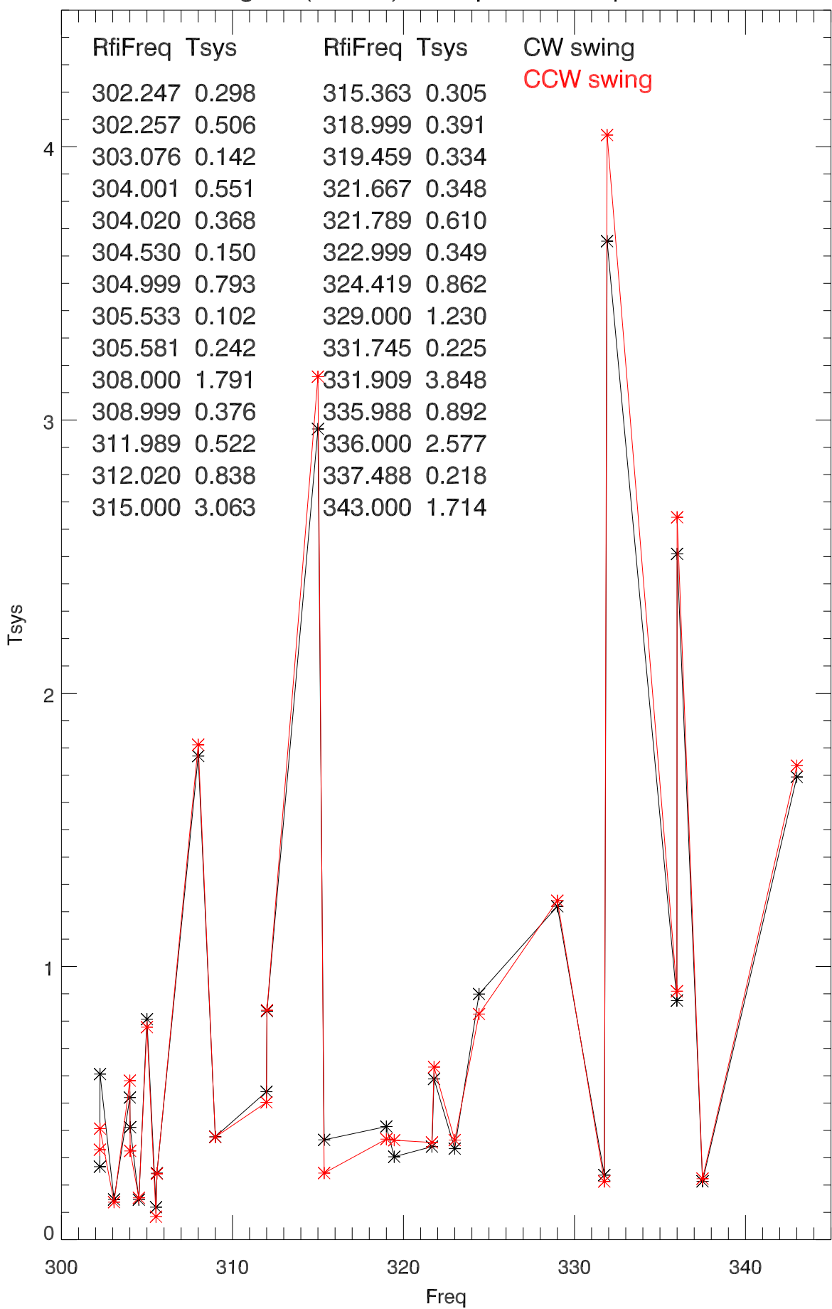
AvgPwr (over az) vs freq for each rfi peak.
