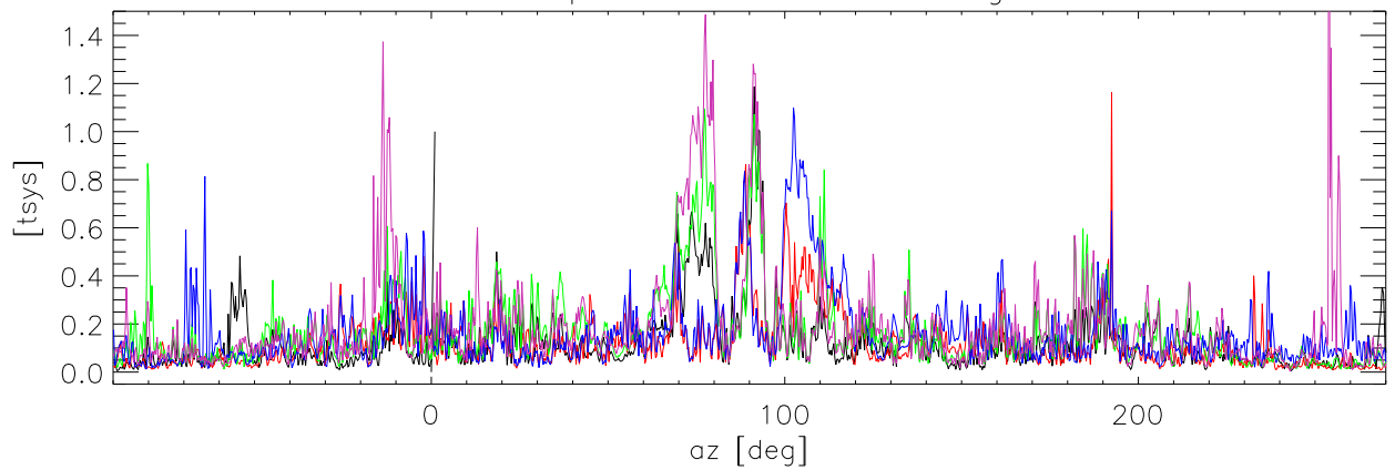
28oct10 319.50 az dependence for 5 az swings. fmstation:106.5
