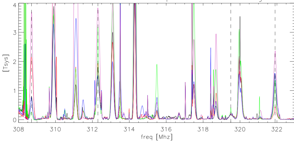
28oct05 327_rcvr max hold spectra for each az swing
