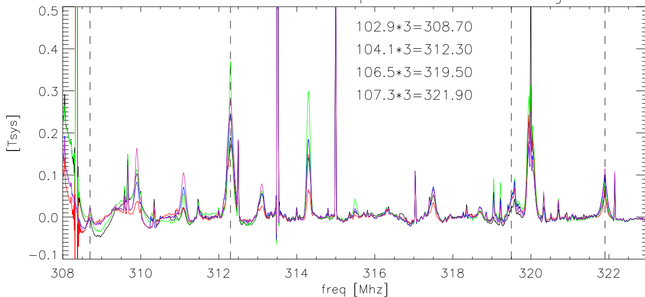
28oct05 327_rcvr median spectra for each az swing
