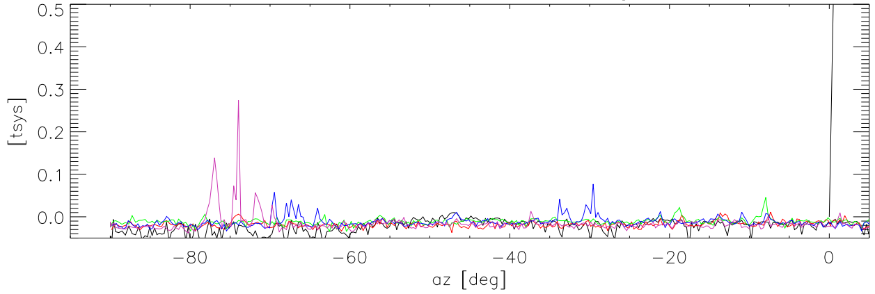
28oct10 308.70 az dependence for 5 az swings. fmstation:102.9
