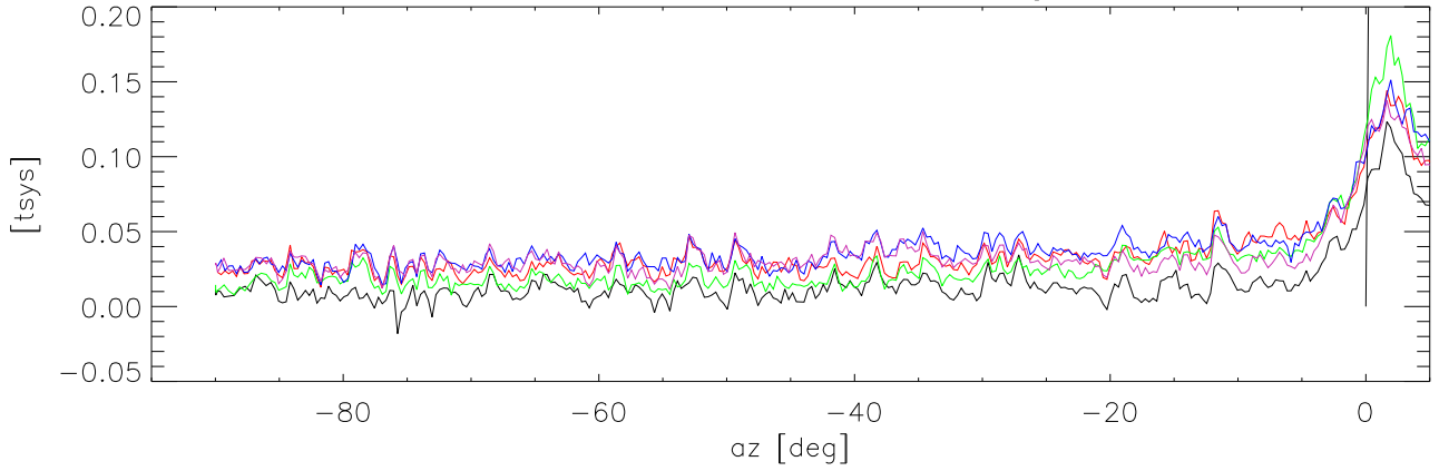
28oct10 319.50 az dependence for 5 az swings. fmstation:106.5
