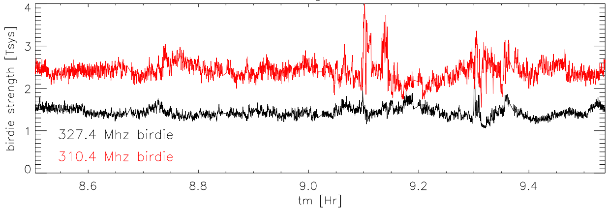
11oct05 327 Freq of 327.4 Mhz birdie vs time
