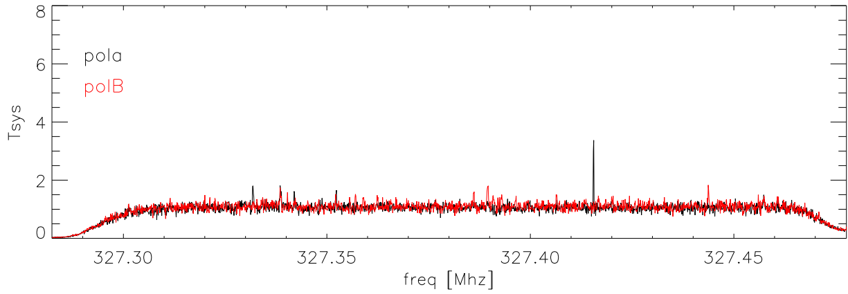
12oct05 310.4 birdie from Ac
