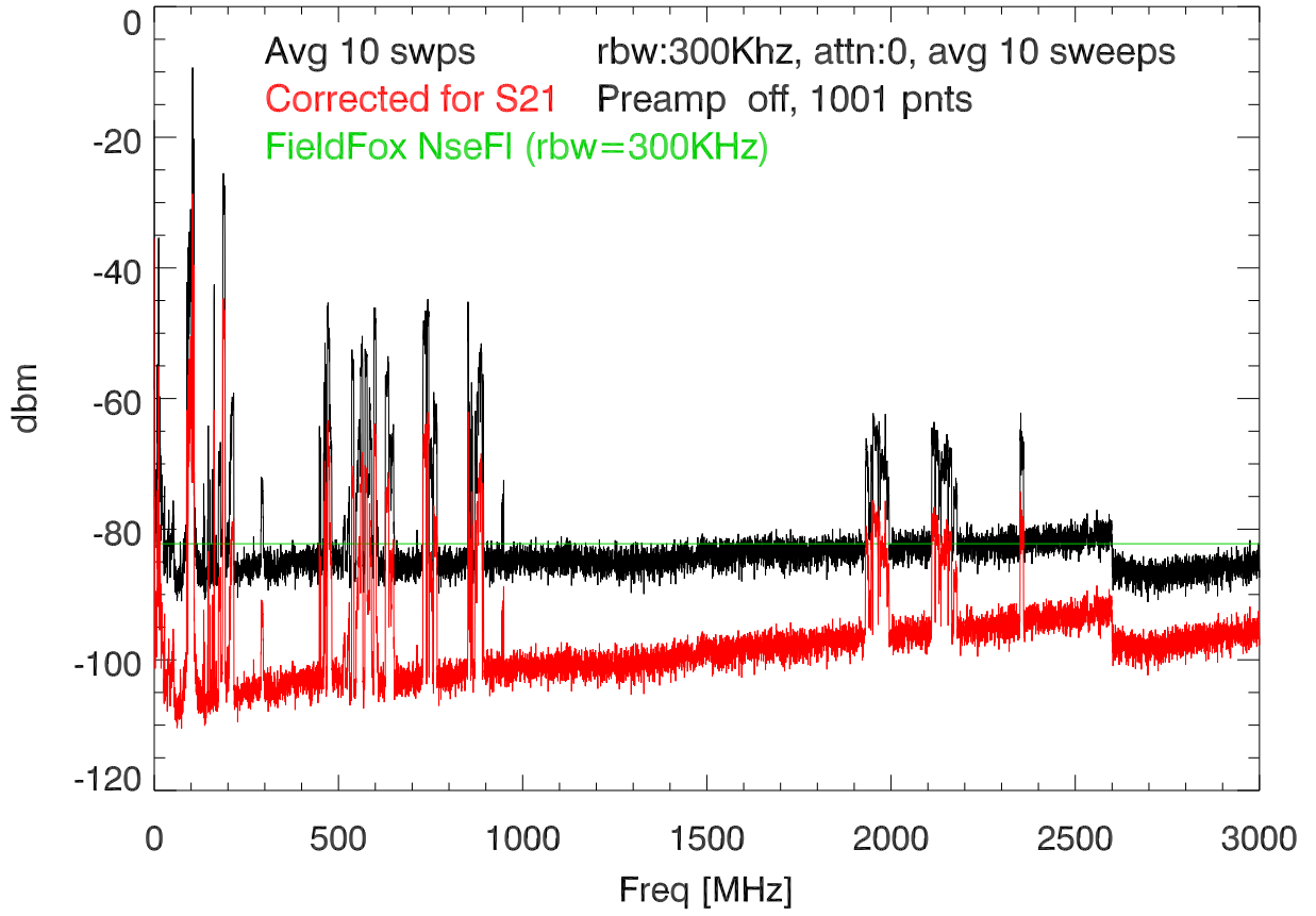
10may21 Input and S21 corrected spectra (FieldFox 9916A)
