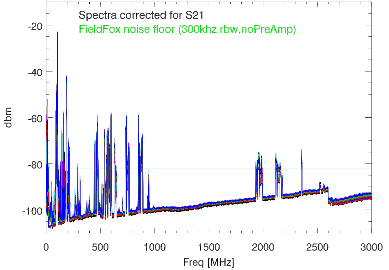
10may21 avg spectra to 1 hour steps: avg spectra
