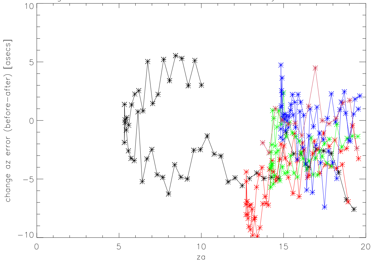
01aug01 sbn. Delta azError vs Za from tertiary motor installation
