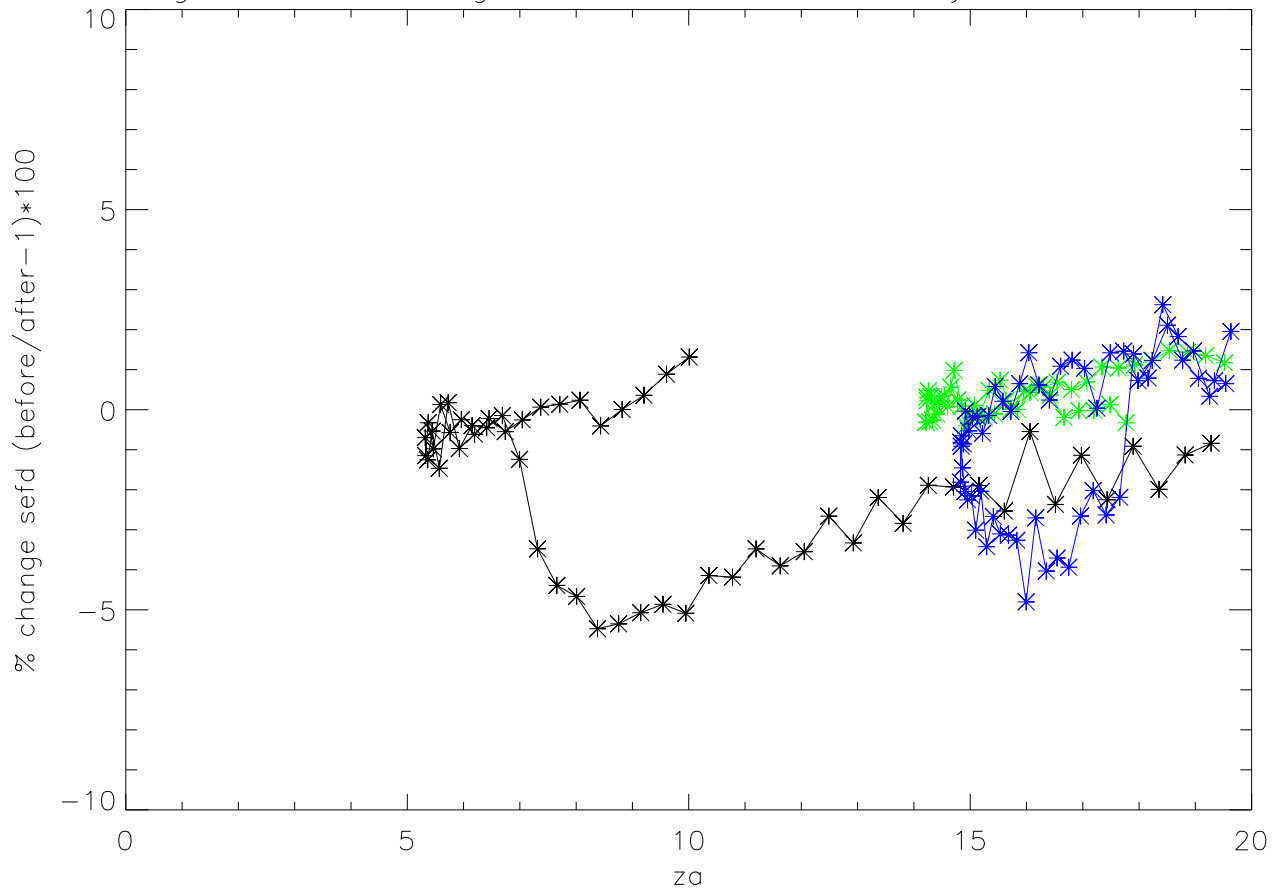
01aug01 sbn. % change SEFD vs Za from tertiary motor installation
