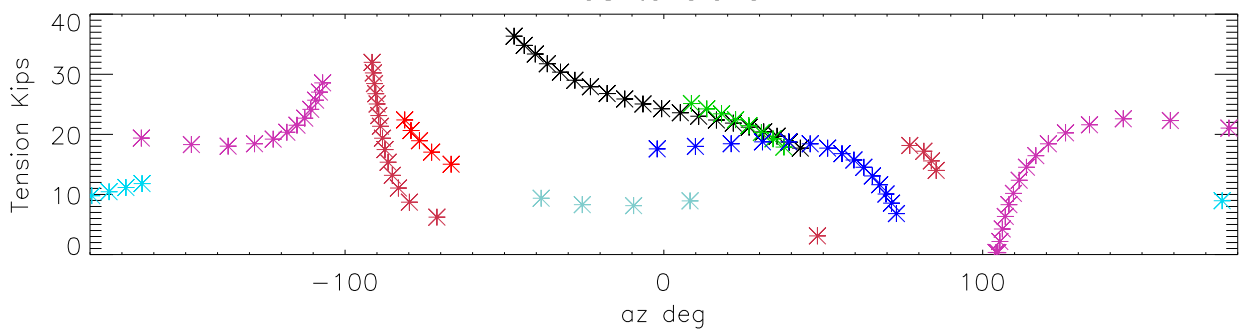
Td8 tensions
