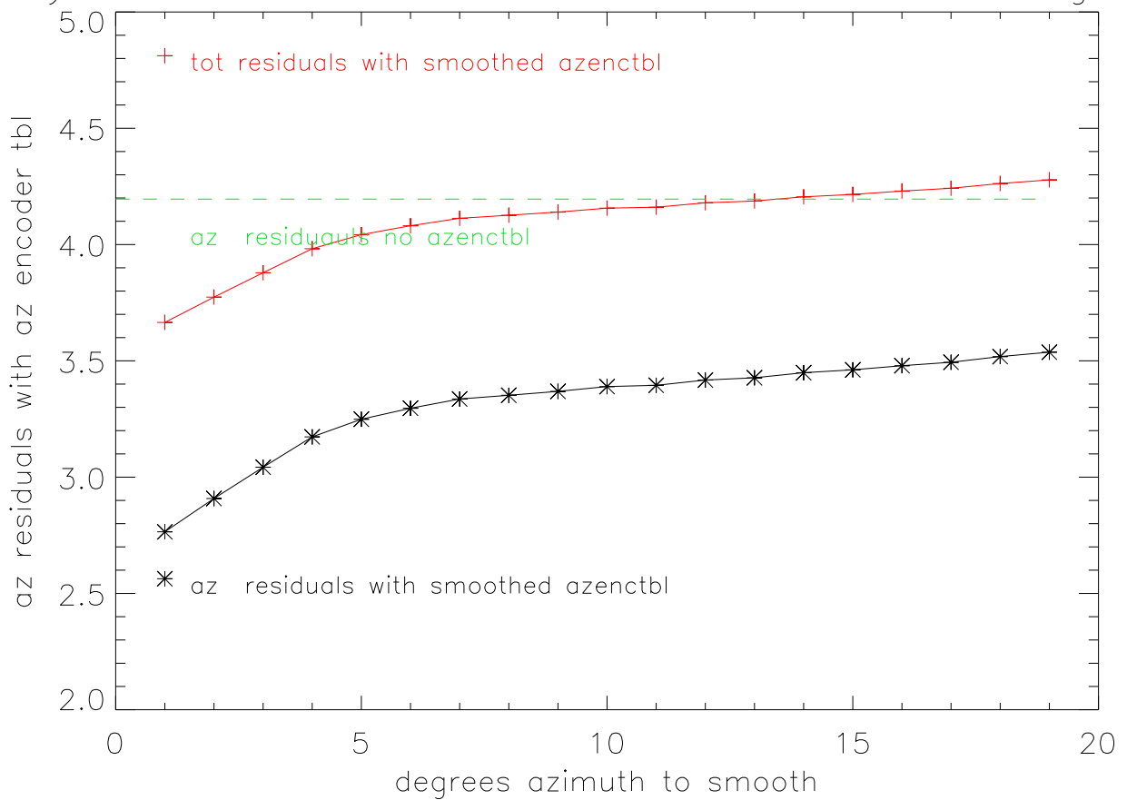
may04 az residuals with encoder table versus smoothing length
