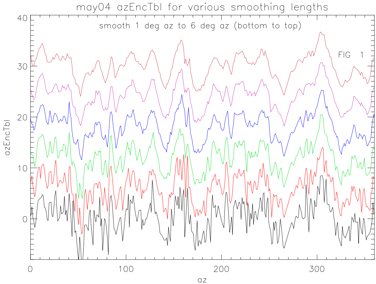
may04 az residuals with encoder table versus smoothing length
