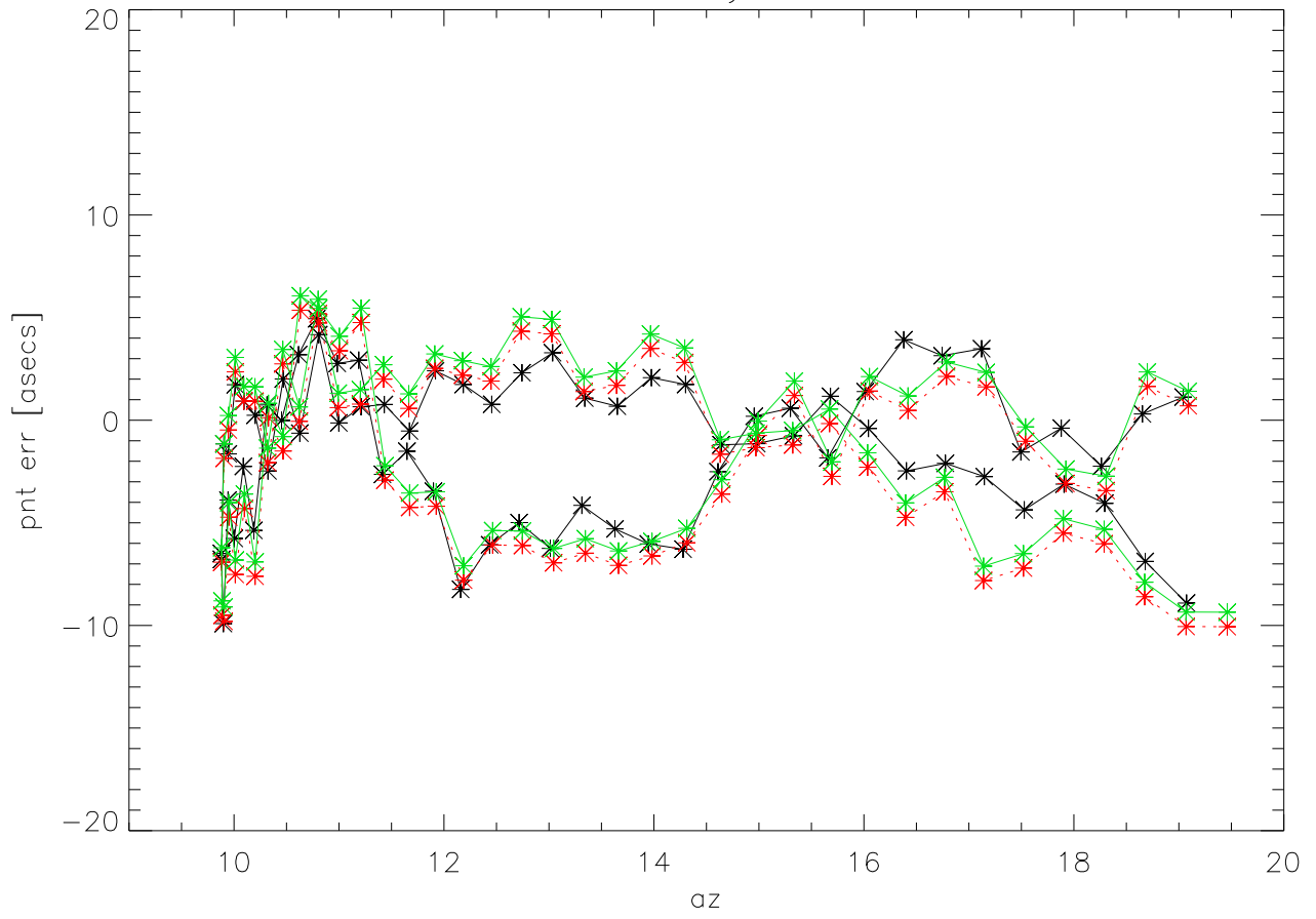
mar03 sbh az verify on J1006+349
