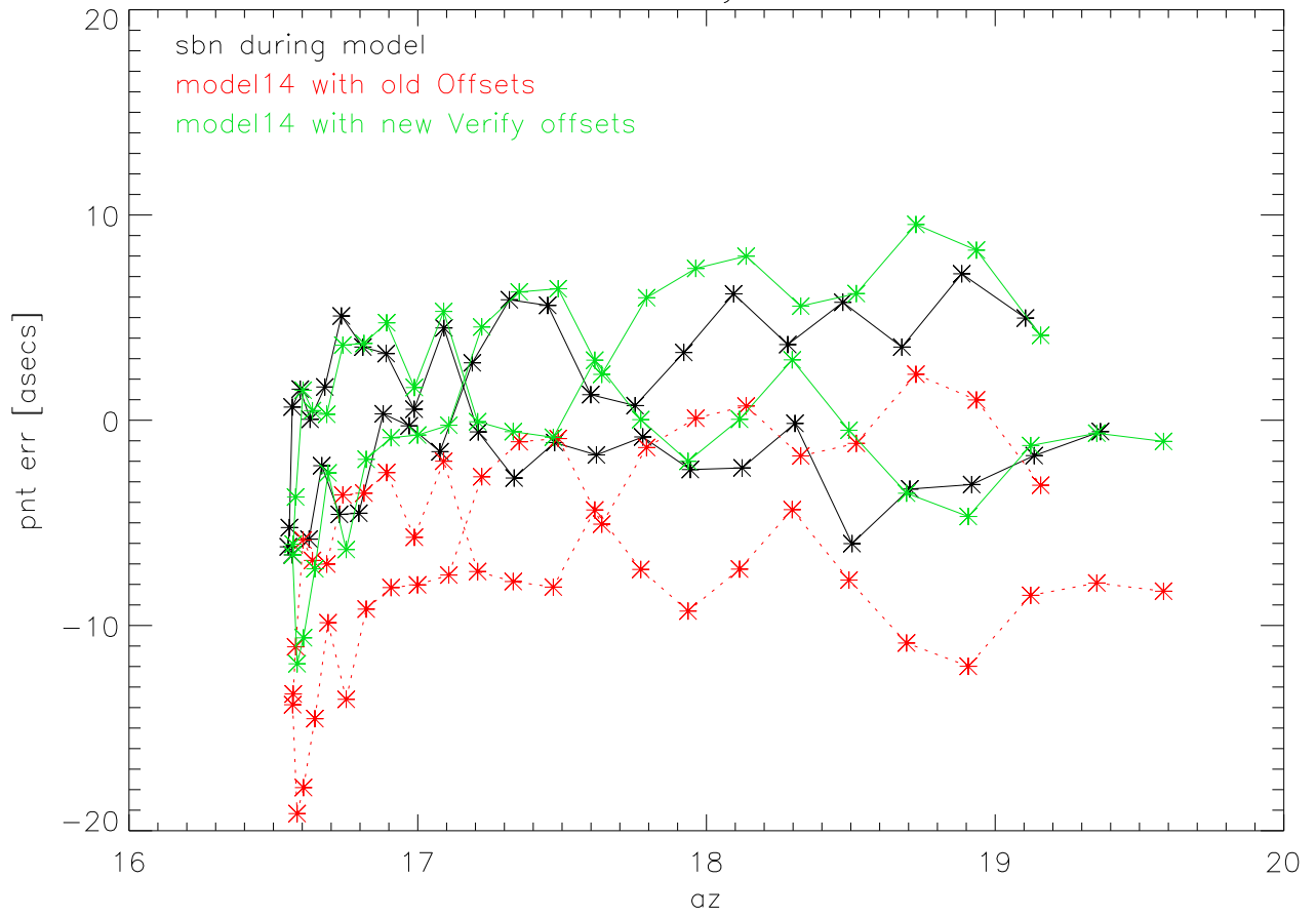
mar03 lbw az verify on J2021+233
