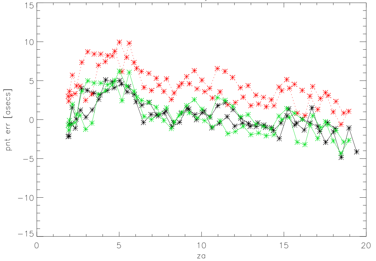
mar03 xband za verify on J0738+177
