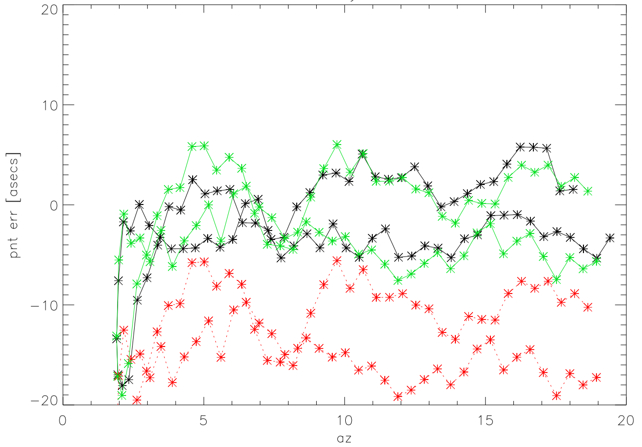
mar03 xband az verify on J0738+177
