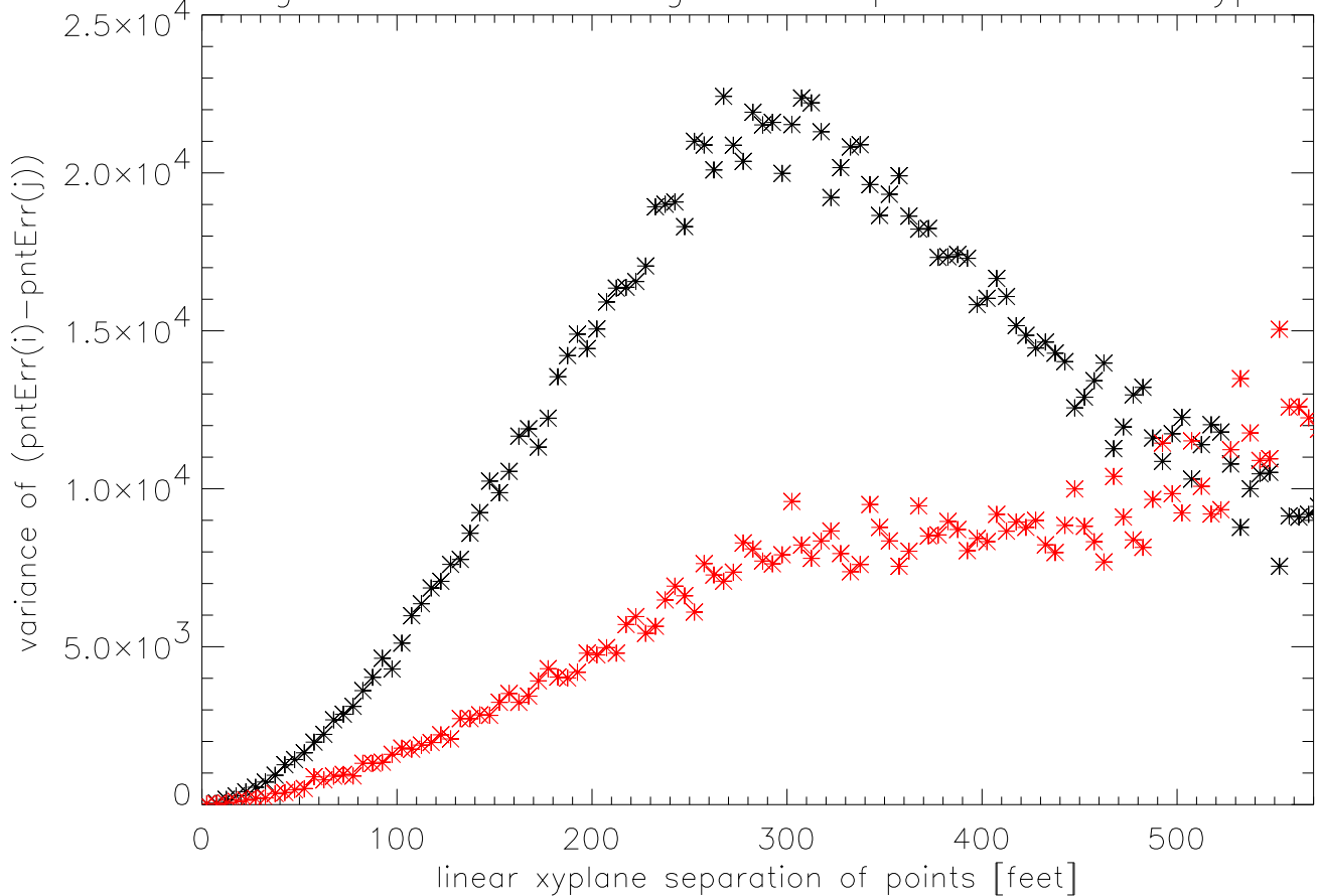
variogram of raw Pointing errors input to model14 xyplane
