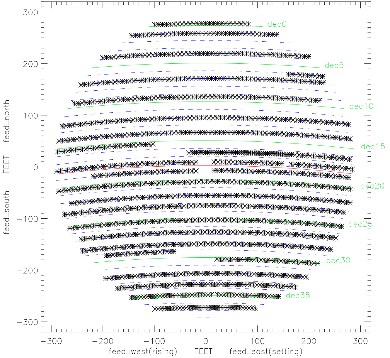
mar03 model 14 az,za coverage
