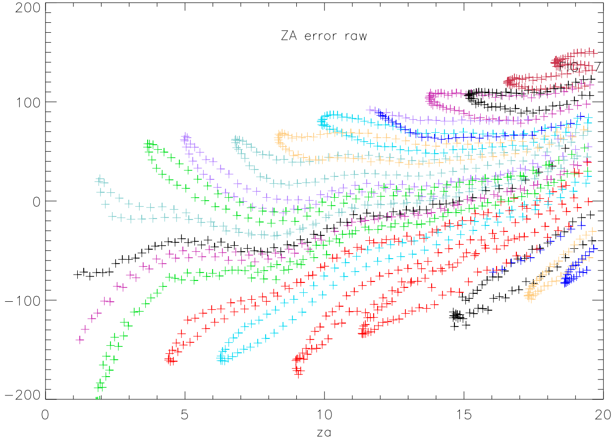
mar03 model 14 raw pointing errors [asecs] az,za vs za
