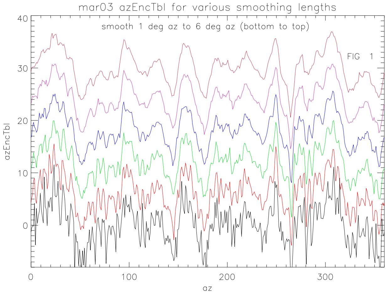
mar03 az residuals with encoder table versus smoothing length
