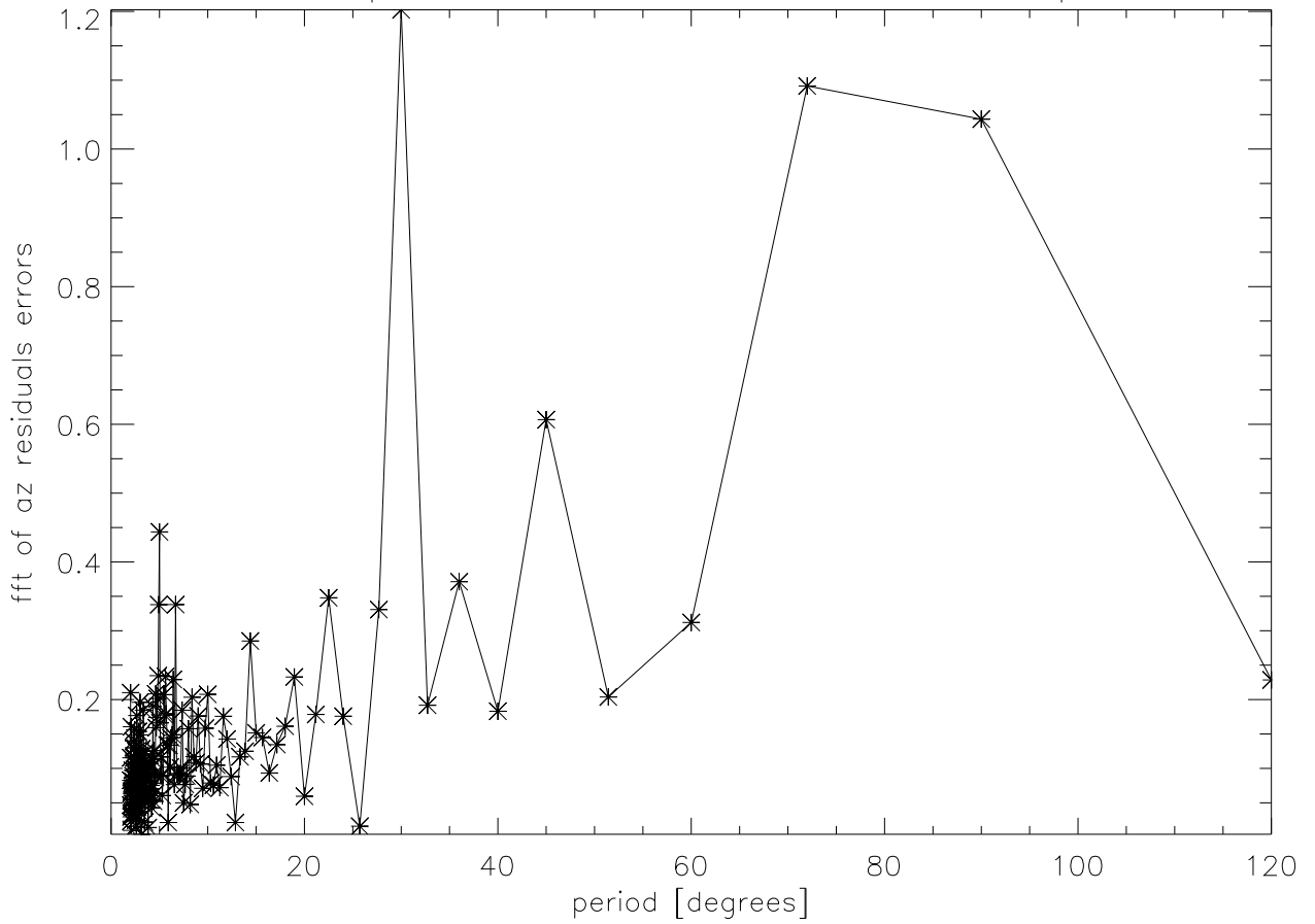
mar03 spectrum of az residual errors versus period
