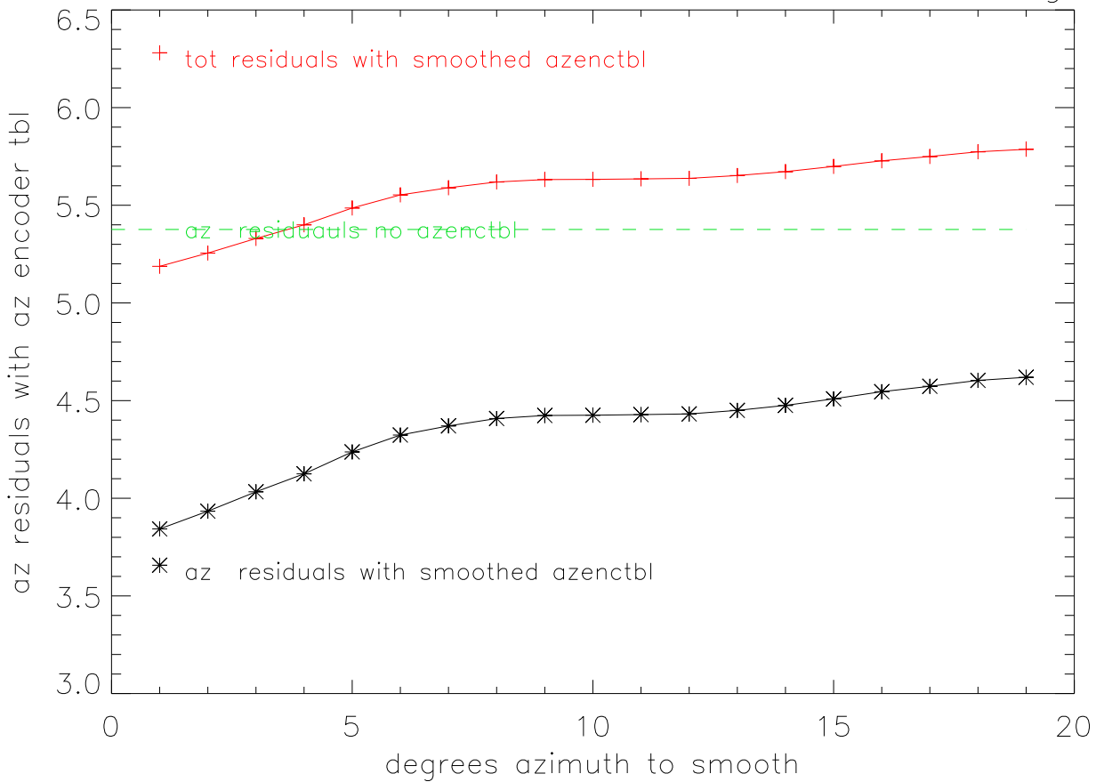
mar03 az residuals with encoder table versus smoothing length
