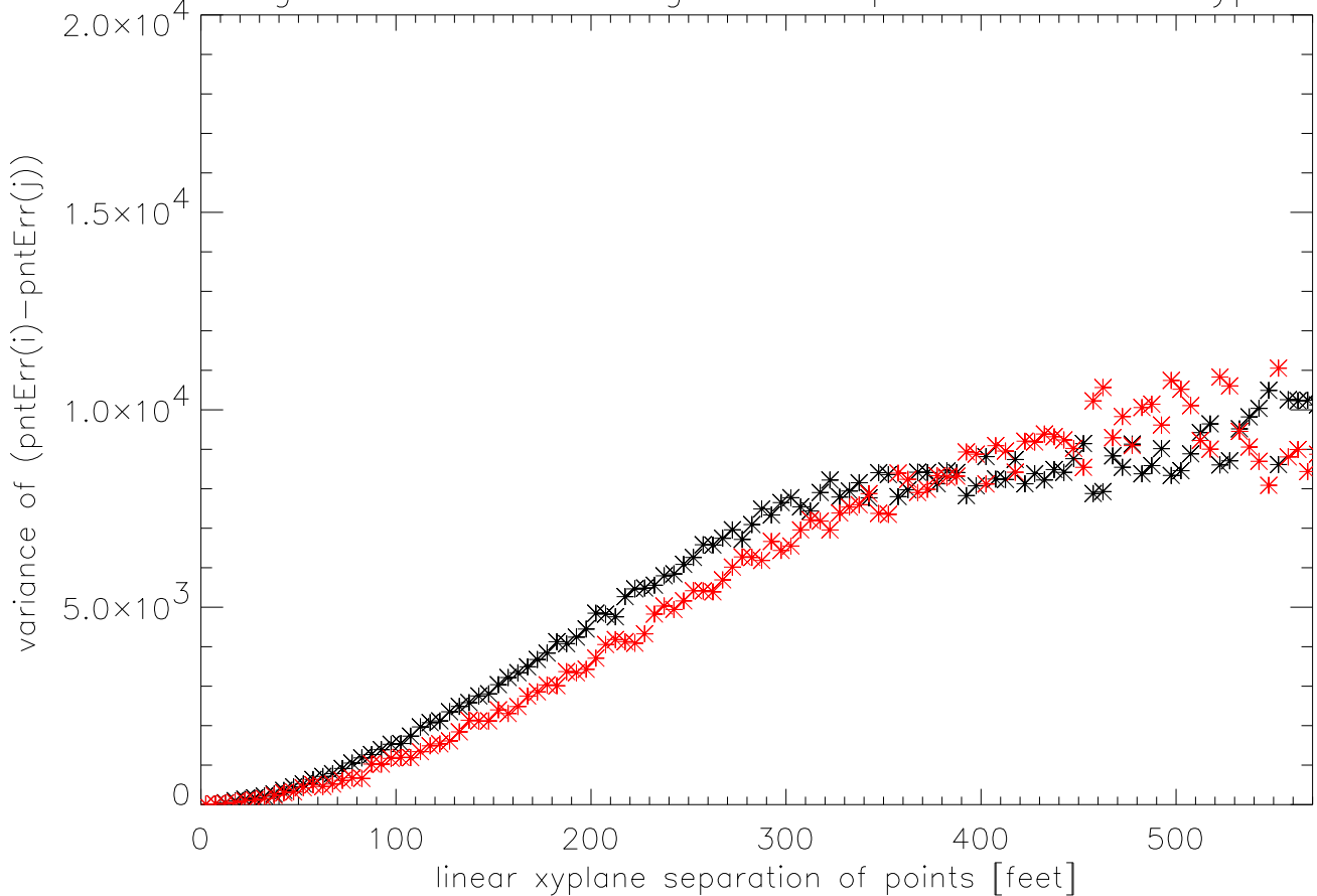
variogram of raw Pointing errors input to model13 xyplane
