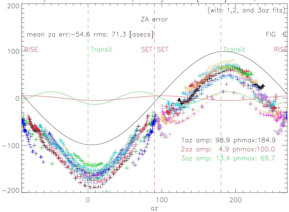
jan02 model 13 raw pointing errors [asecs] vs az,za
