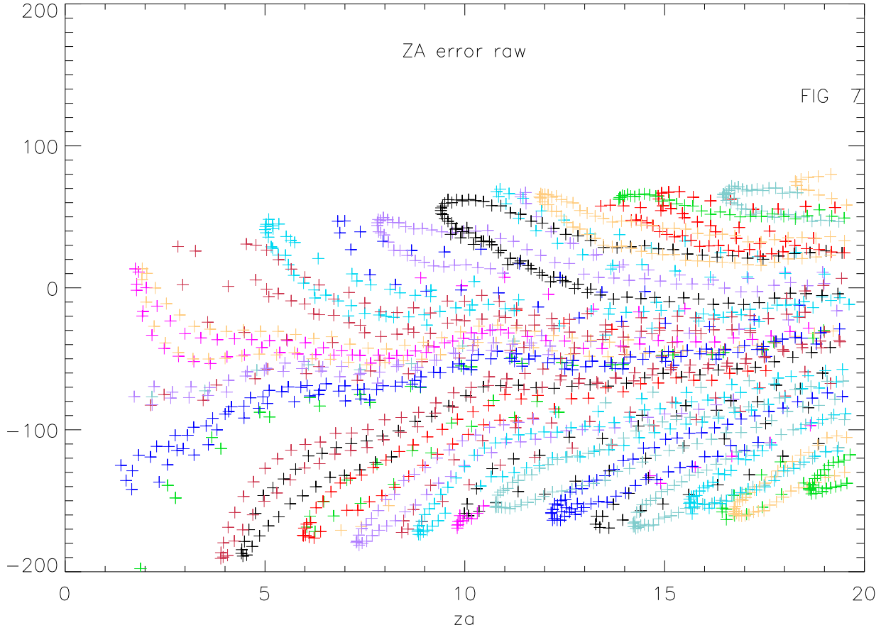
jan02 model 13 raw pointing errors [asecs] az,za vs za
