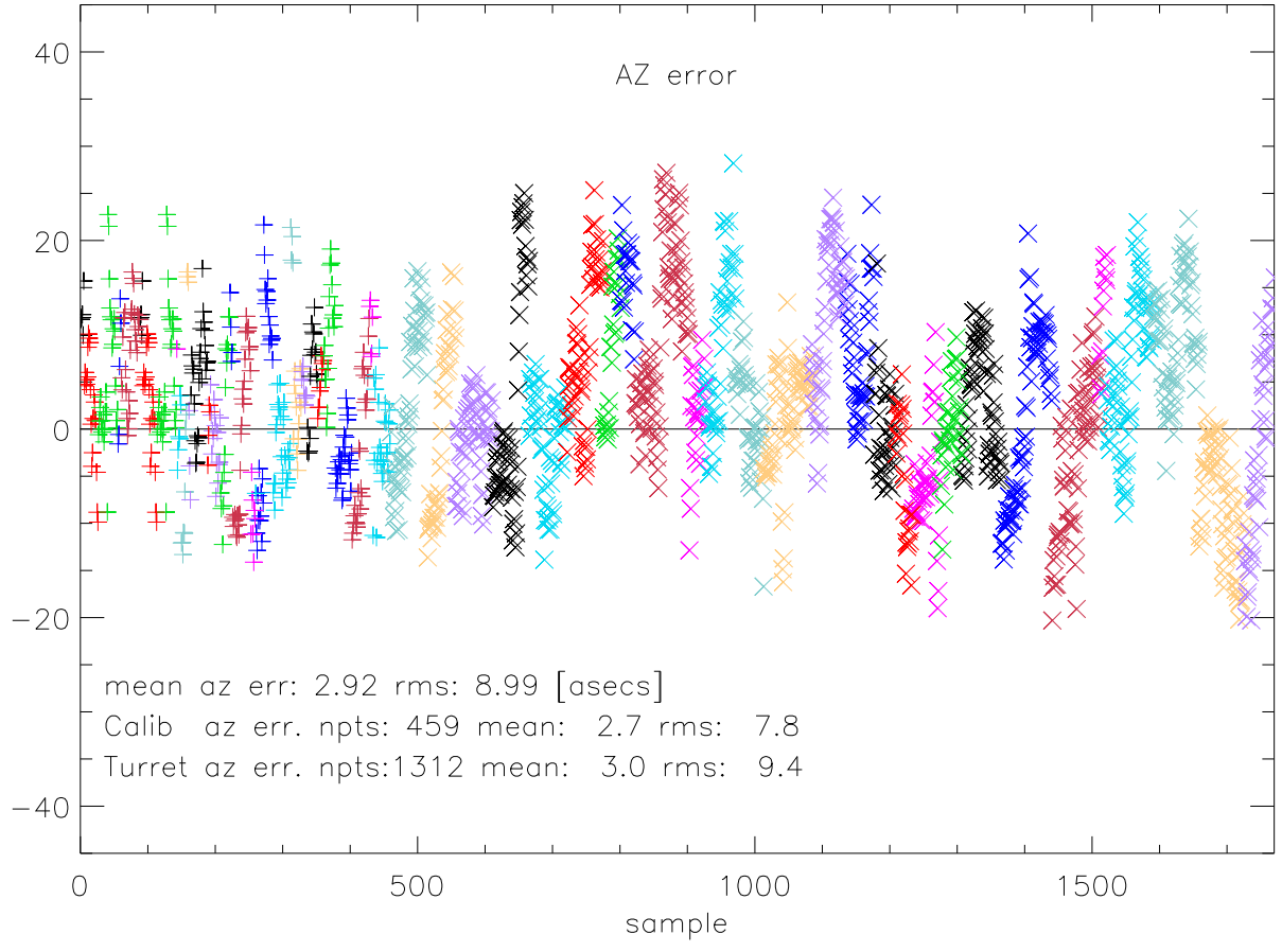
azimuth error [asecs] relative to model 11 by src
