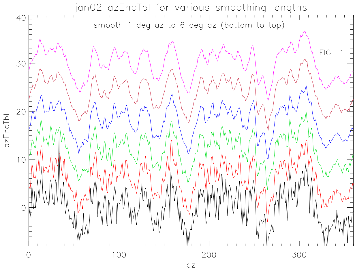
jan02 az residuals with encoder table versus smoothing length
