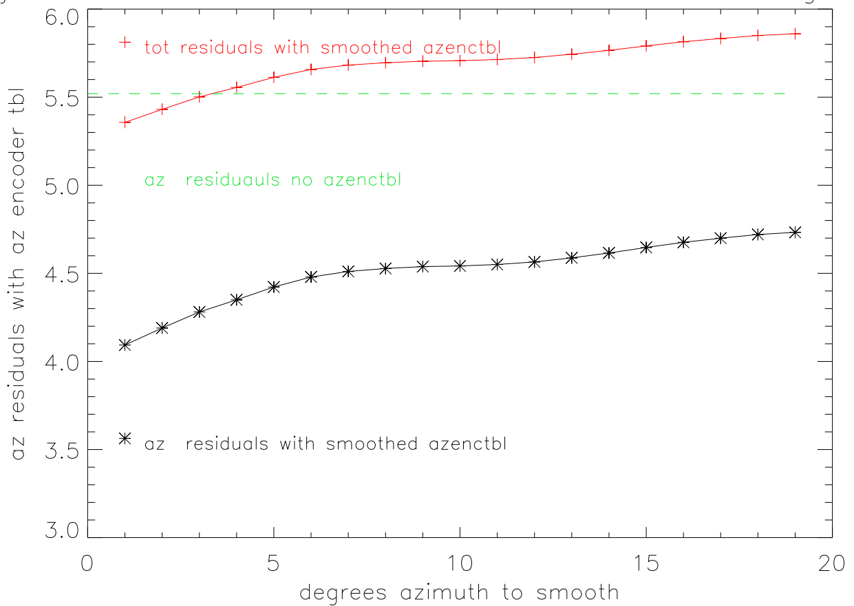
jan02 az residuals with encoder table versus smoothing length
