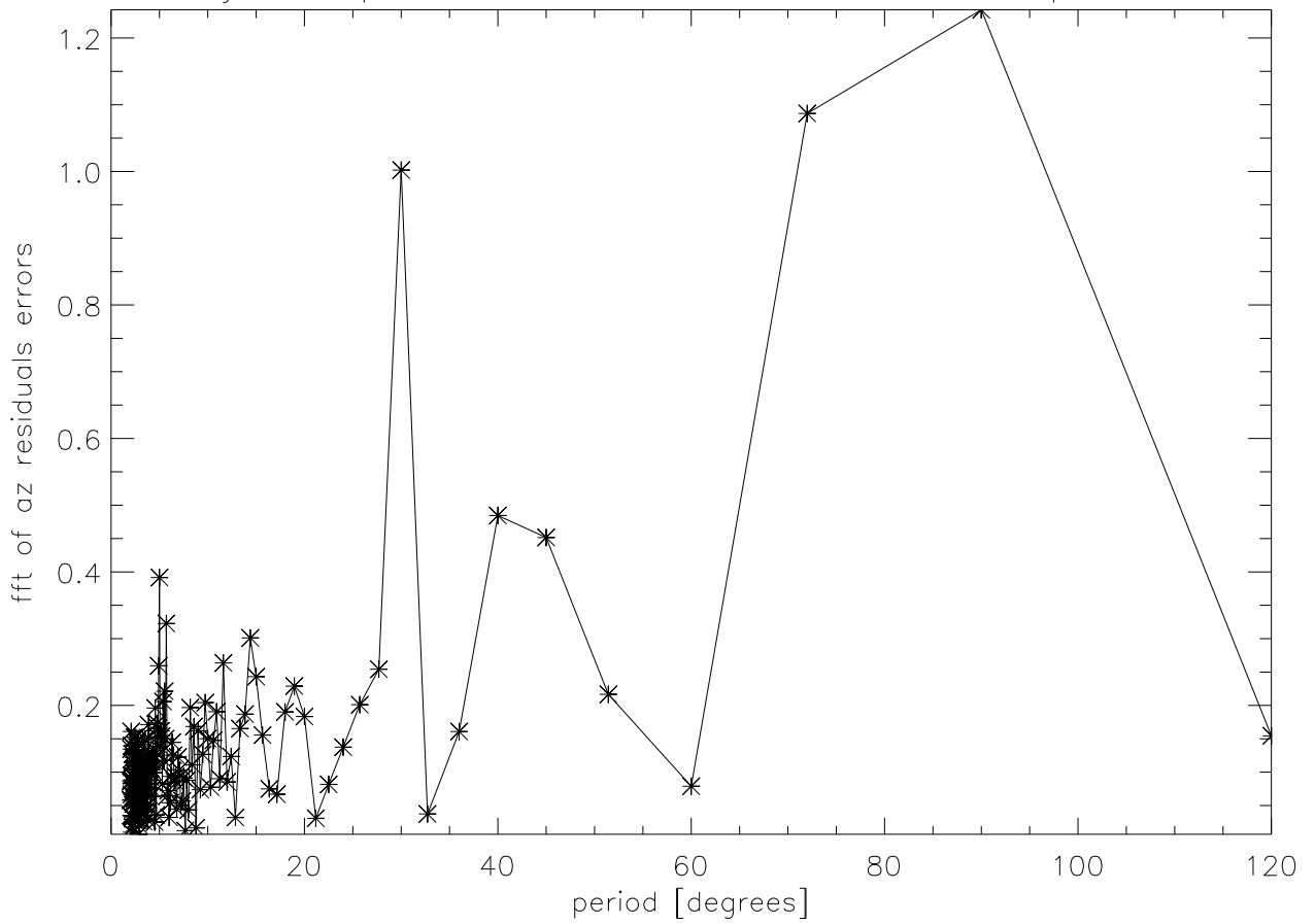
jan02 spectrum of az residual errors versus period
