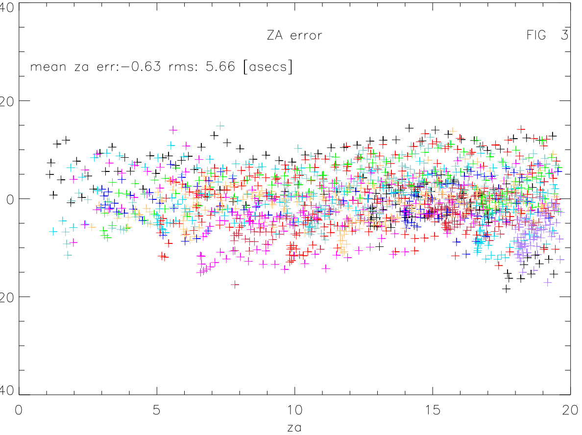
zenith angle, azimuth error [asecs] relative to model 11 versus za
