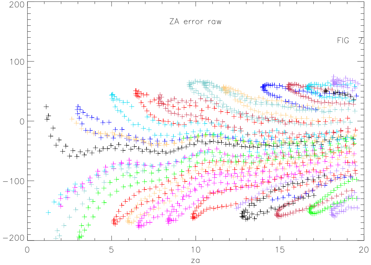
feb01 model 12 raw pointing errors [asecs] az,za vs za
