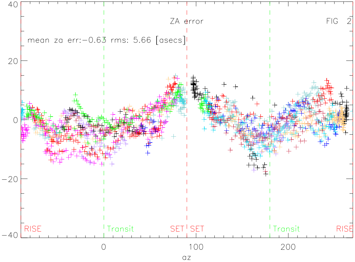
zenith angle, azimuth error [asecs] relative to model 11 versus az
