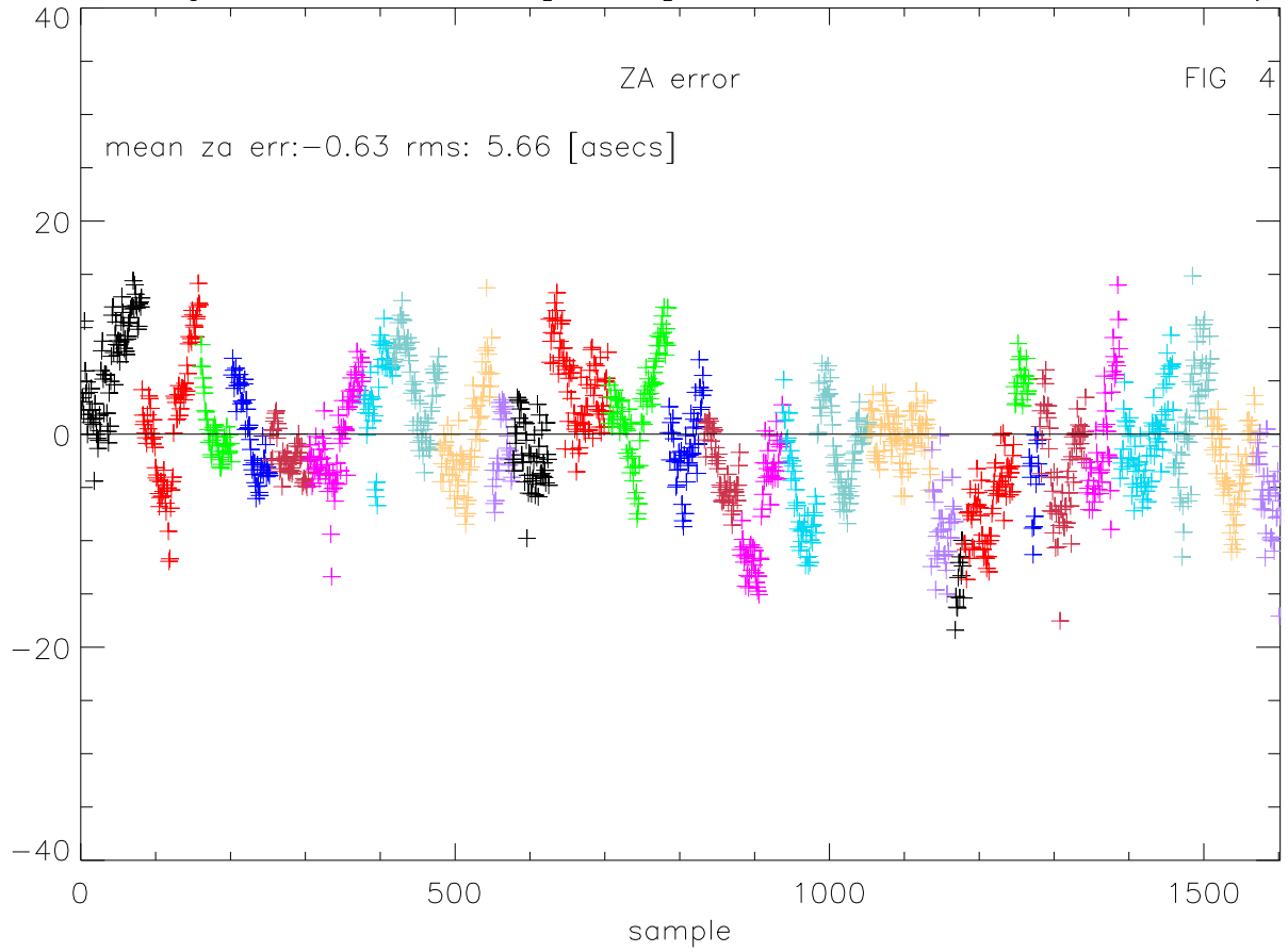
zenith angle, azimuth error [asecs] relative to model 11 versus by src
