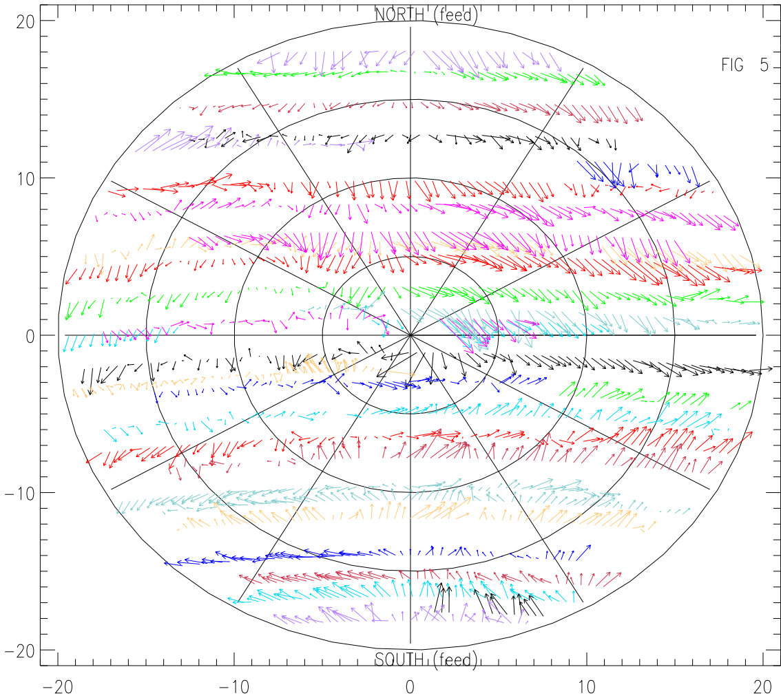
FEB01 pointing errors input to model 12 (relative to model 11) vs az,za 1 div=10.00asecs
