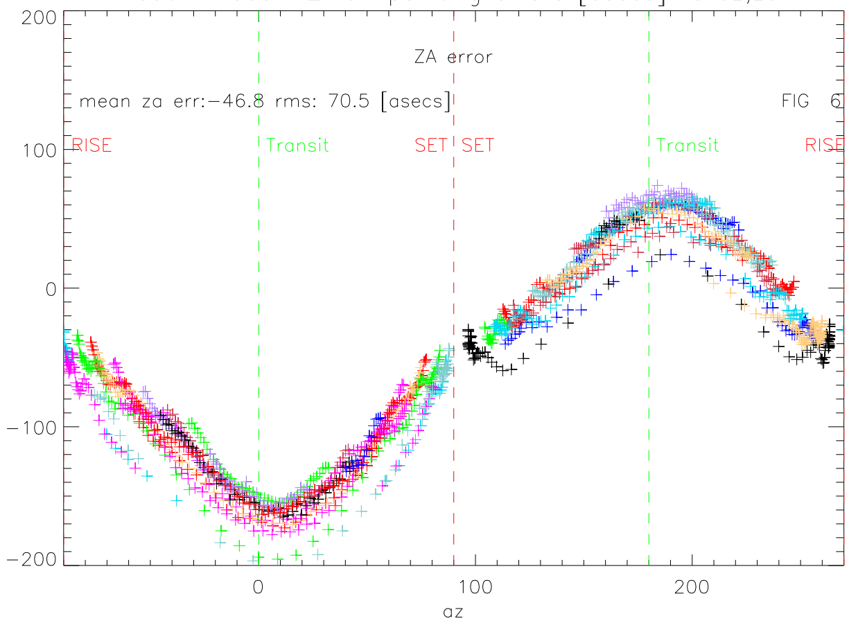
feb01 model 12 raw pointing errors [asecs] vs az,za
