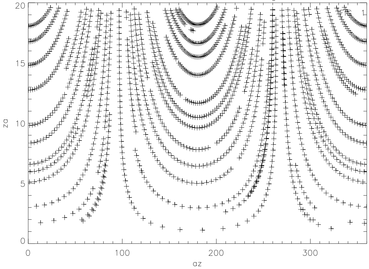
Feb01 model 12 az,za coverage
