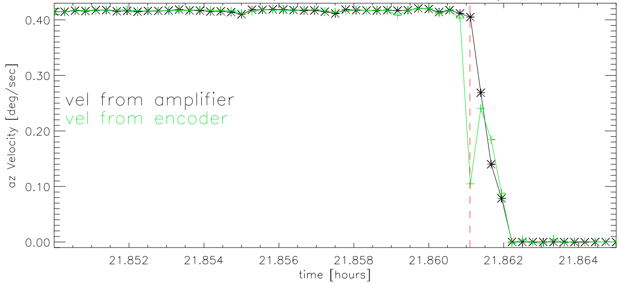
15sep02 Az velocity vs time at azimuth encoder jump
