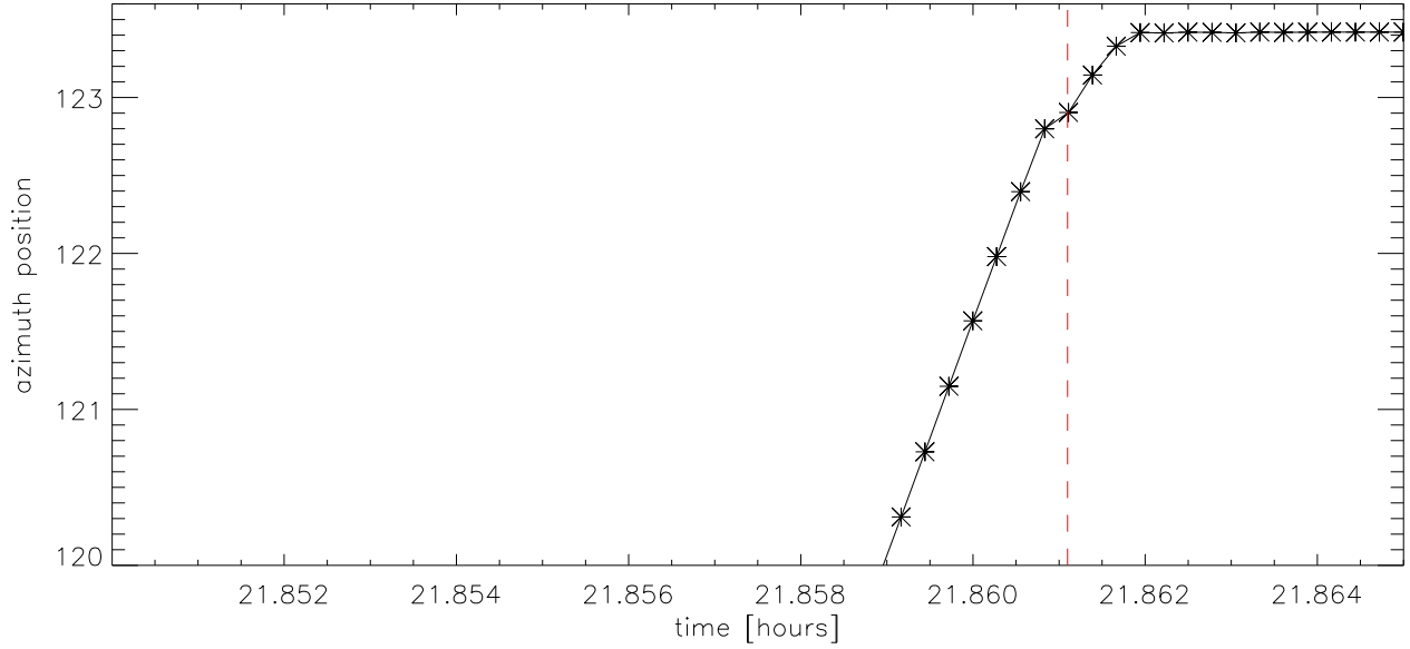
15sep02 Difference azEncoders vs time at azimuth encoder jump
