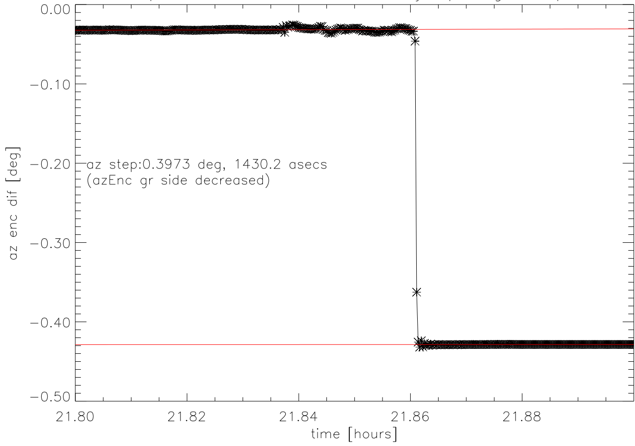
15sep02 linear fits to before,after jump to get StepSize
