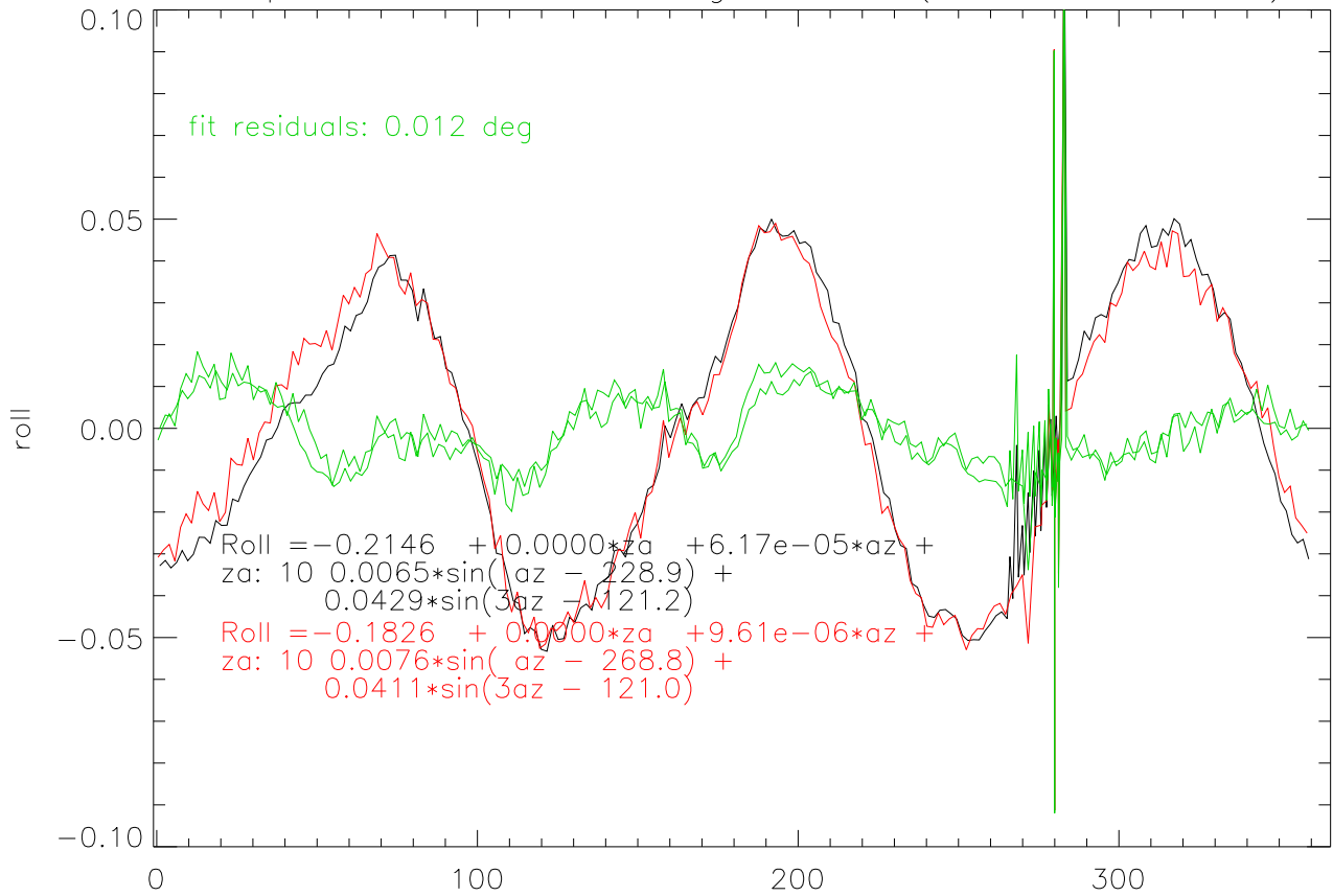
30apr12 tilt sensor az swings Roll - (c0+c1*az from fit)
