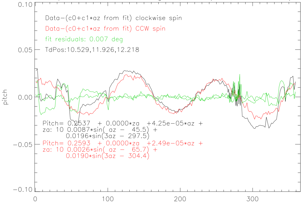
30apr12 tilt sensor az swings PITCH - (c0+c1*az from fit)
