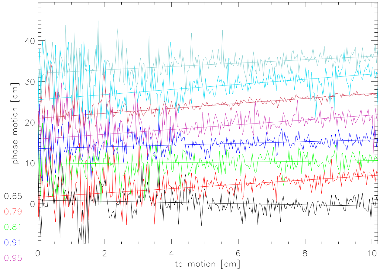
phase motion [cm] vs td motion for 7 peaks (moving up)
