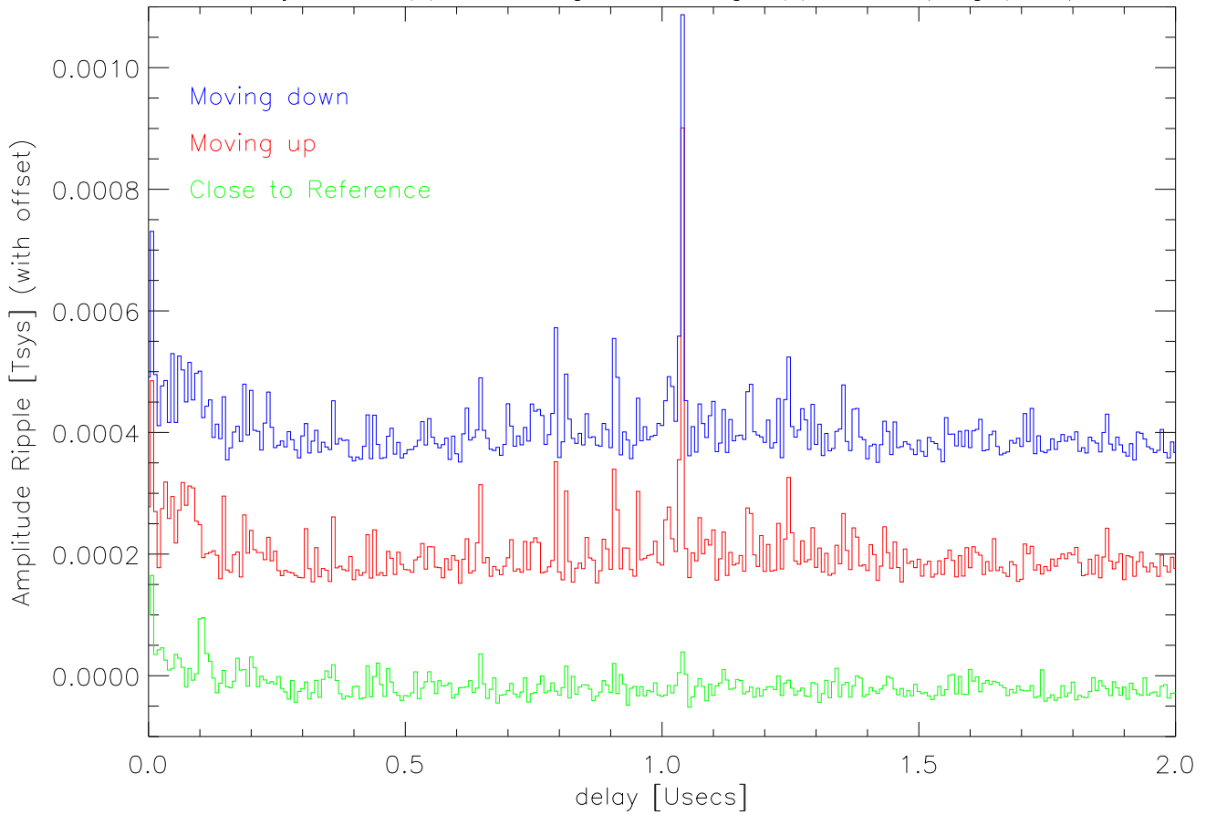
04jan05 Ripple strength (average polys and direction)
