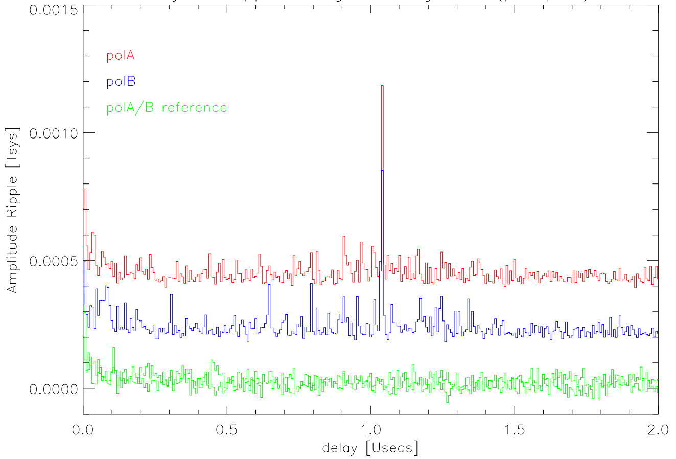
04jan05 Average Strength ripples moving Up
