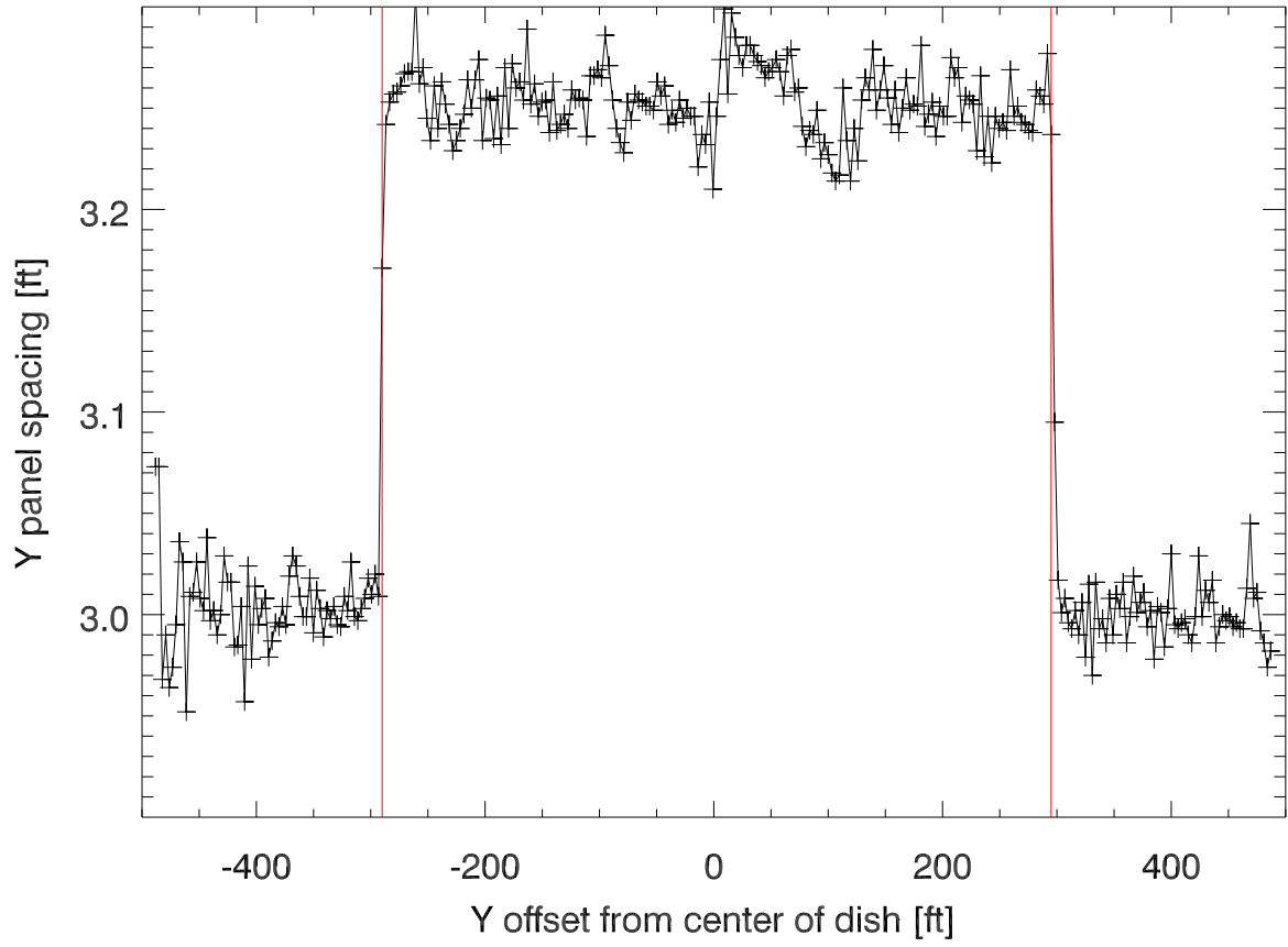
Median (along each E/W cable) Y panel spacing vs Y offset
