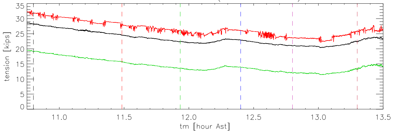
tiedown cable tensions (sum of 2 cables)
