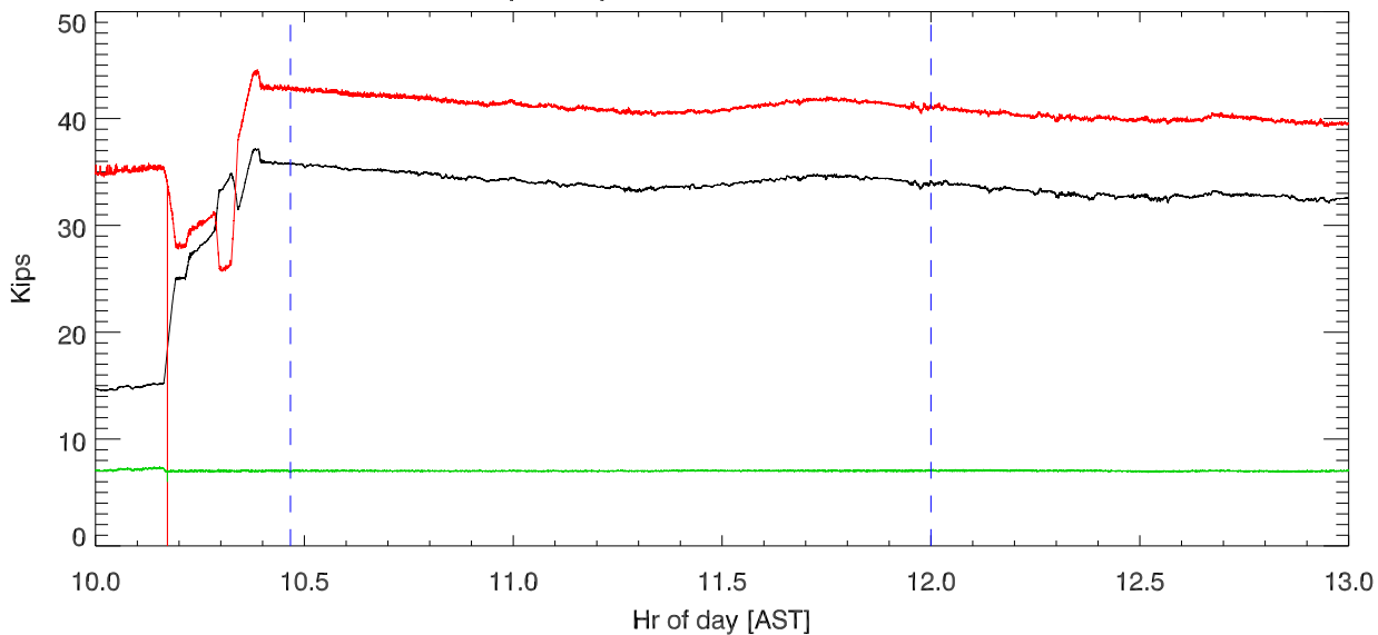
Kips on platform corners from tds
