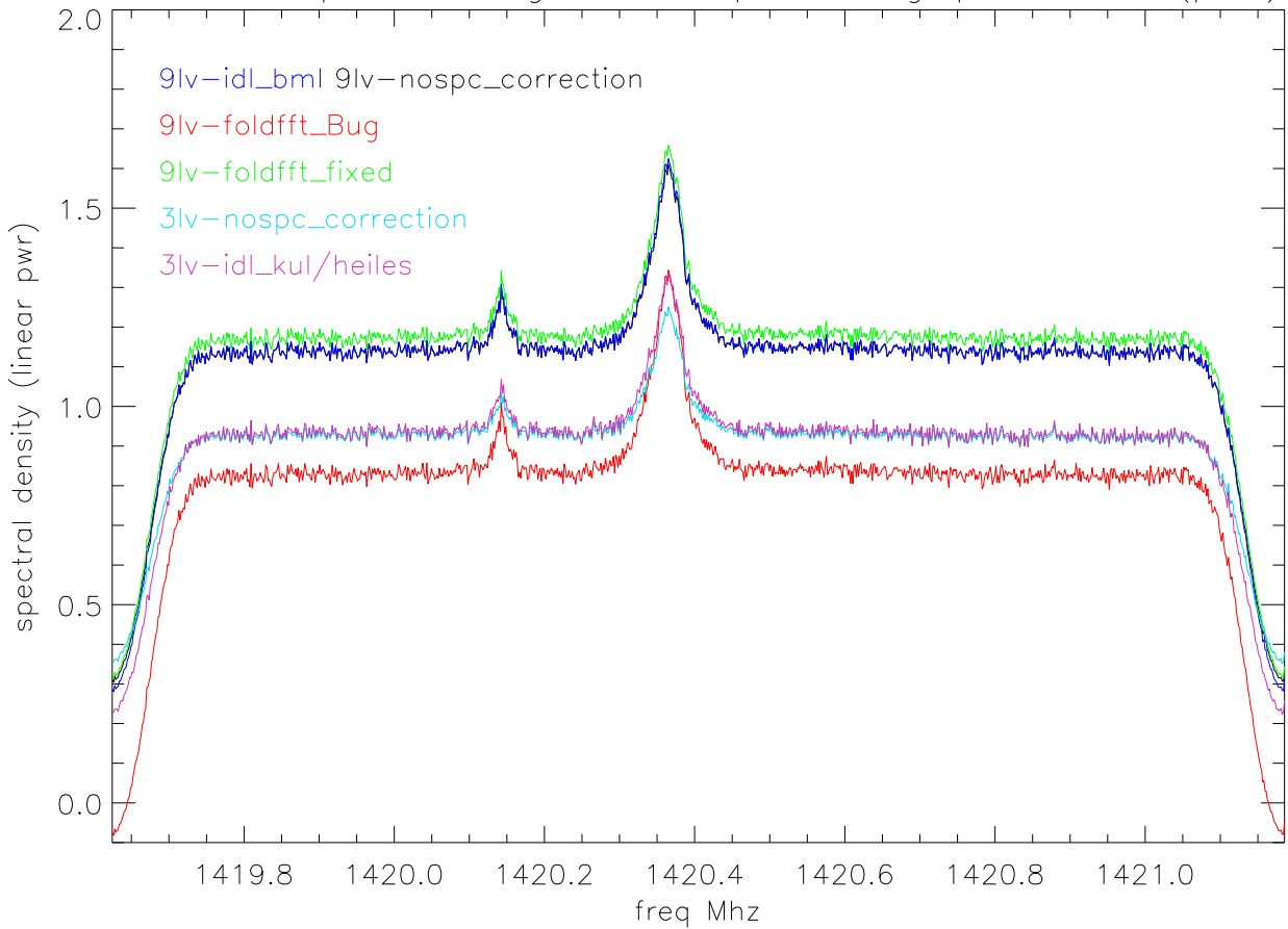
0950+08 spectra using different processing. phaseBin 0 (polA)
