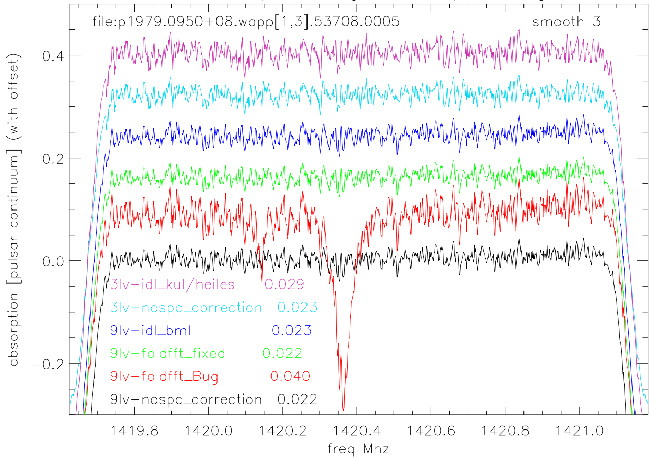
0950+08 spectra using different processing. phaseBin 0 (polA)
