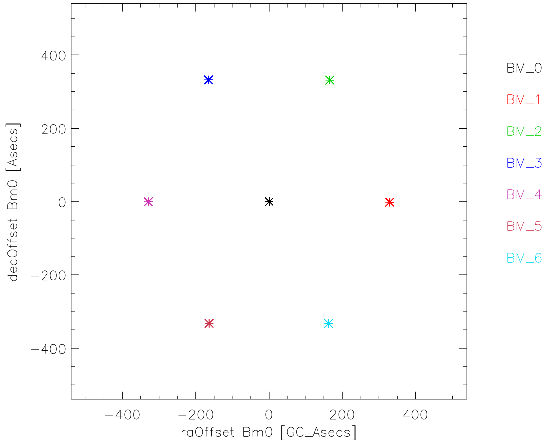
mock J2109+355 alfaAng=-60
