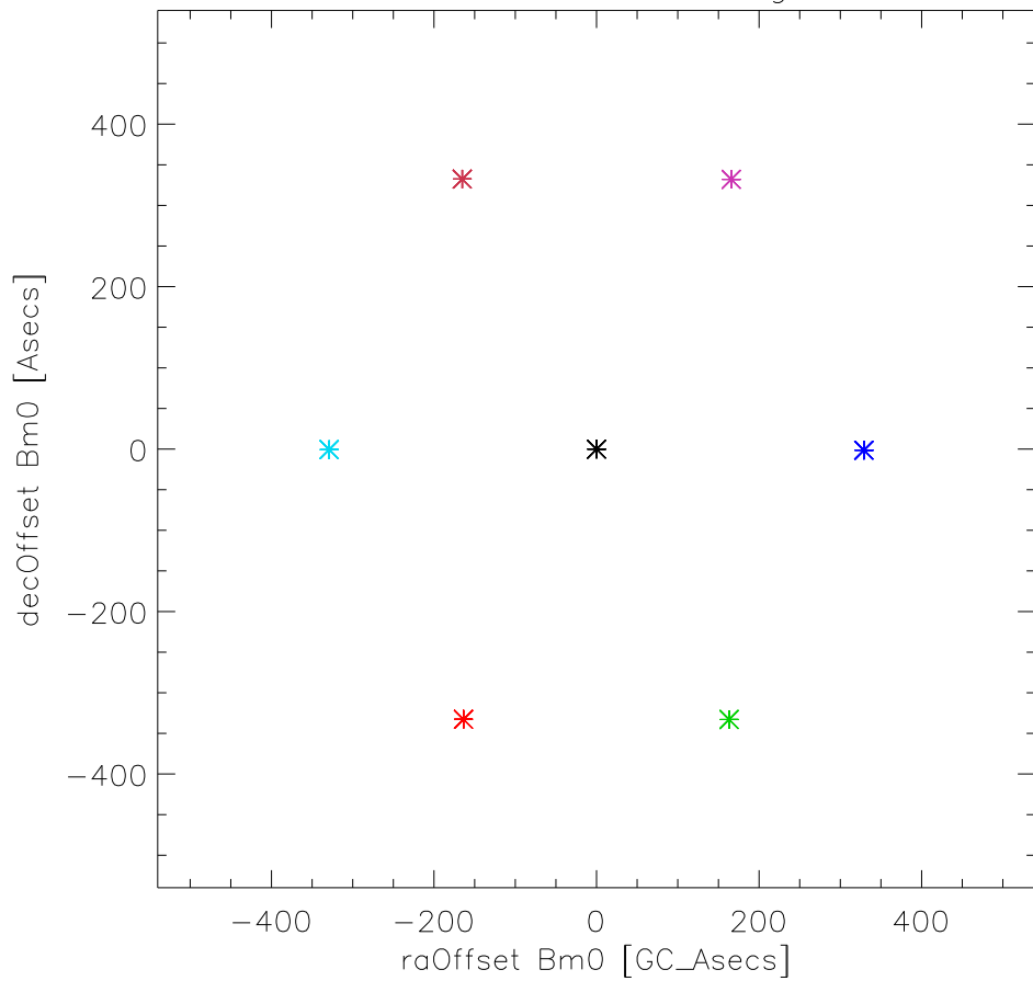
mock J2109+355 alfaAng=-60
