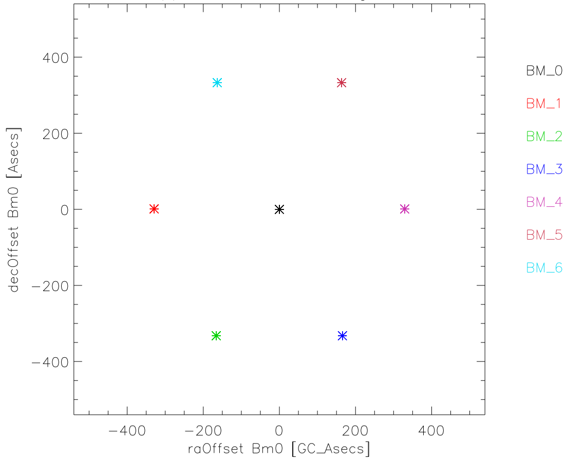
mock J2130+050 alfaAng=-60
