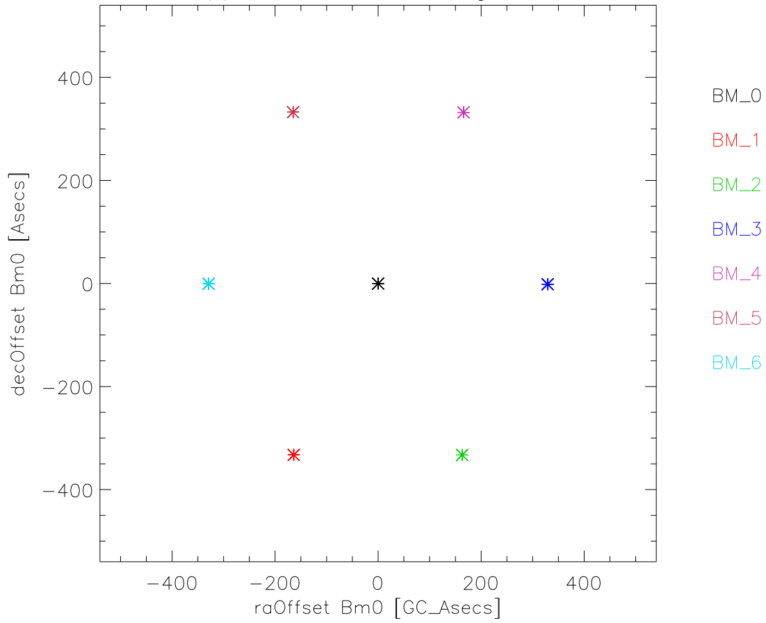
mock J2052+365 alfaAngle=+60
