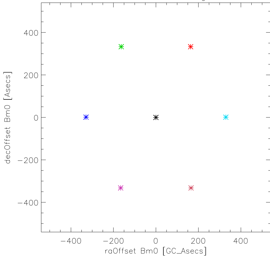
mock J2130+050 alfaAng=-60
