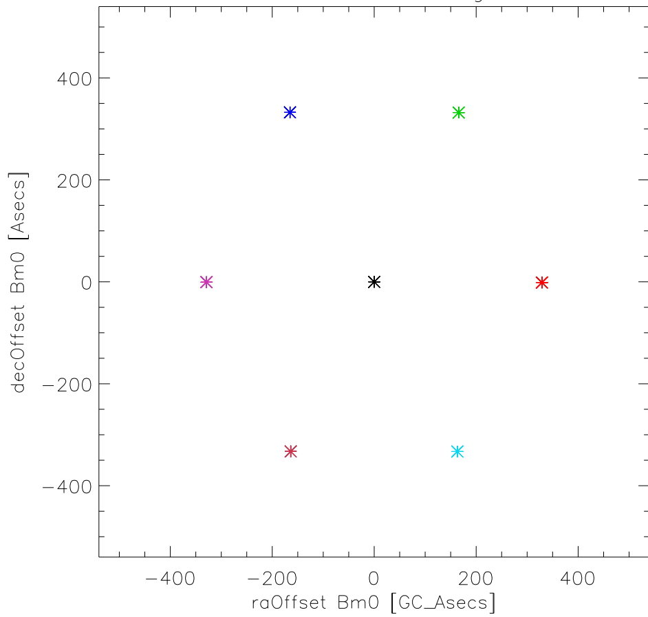
mock J2052+365 alfaAngle=+60
