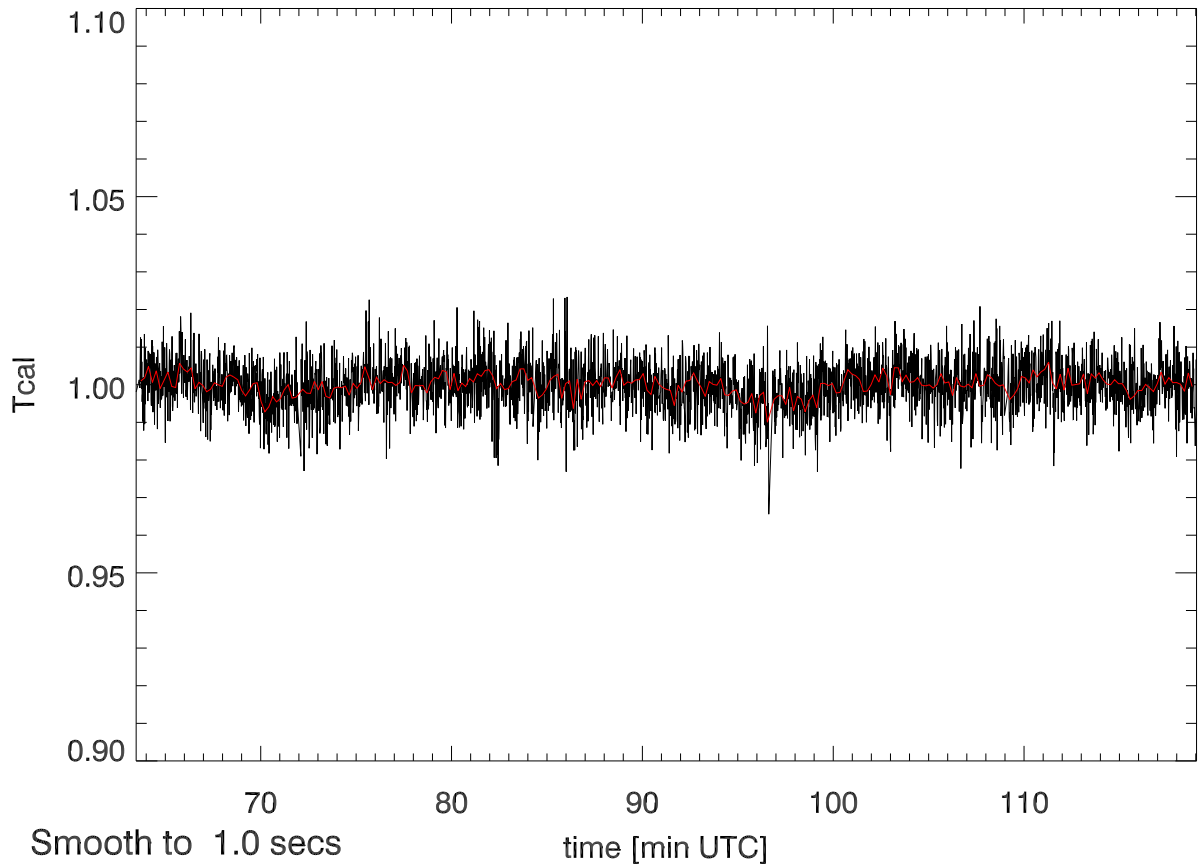
29dec15 calOn - calOff Beam4A SigA: 0.012
