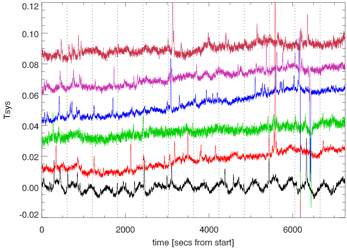
19apr11:alfa a2010 total power vs time for 13 600 sec scans. PoIA
