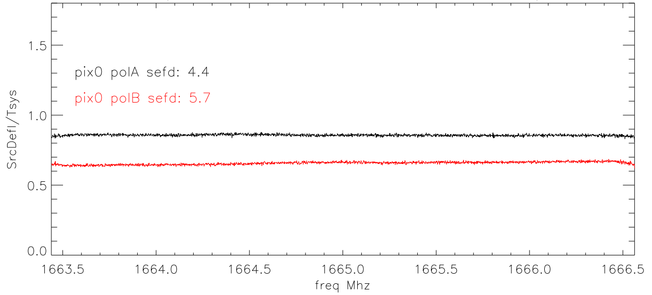
Alfa Pixel 1 SrcDeflection/Tsys
