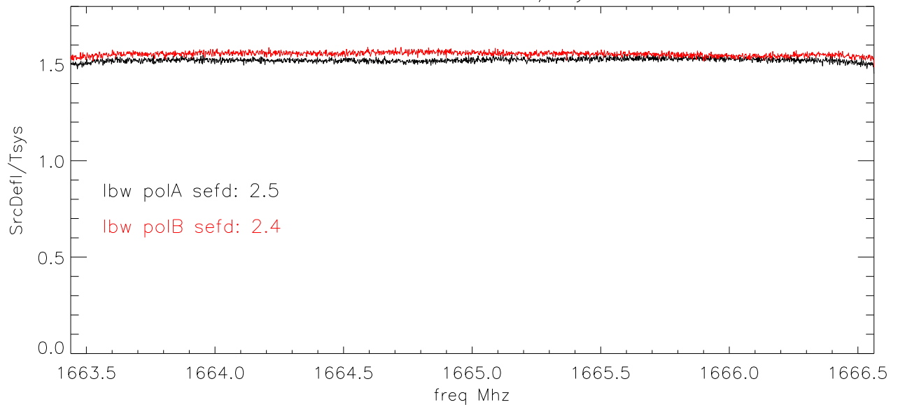
Lbw SrcDeflection/Tsys
