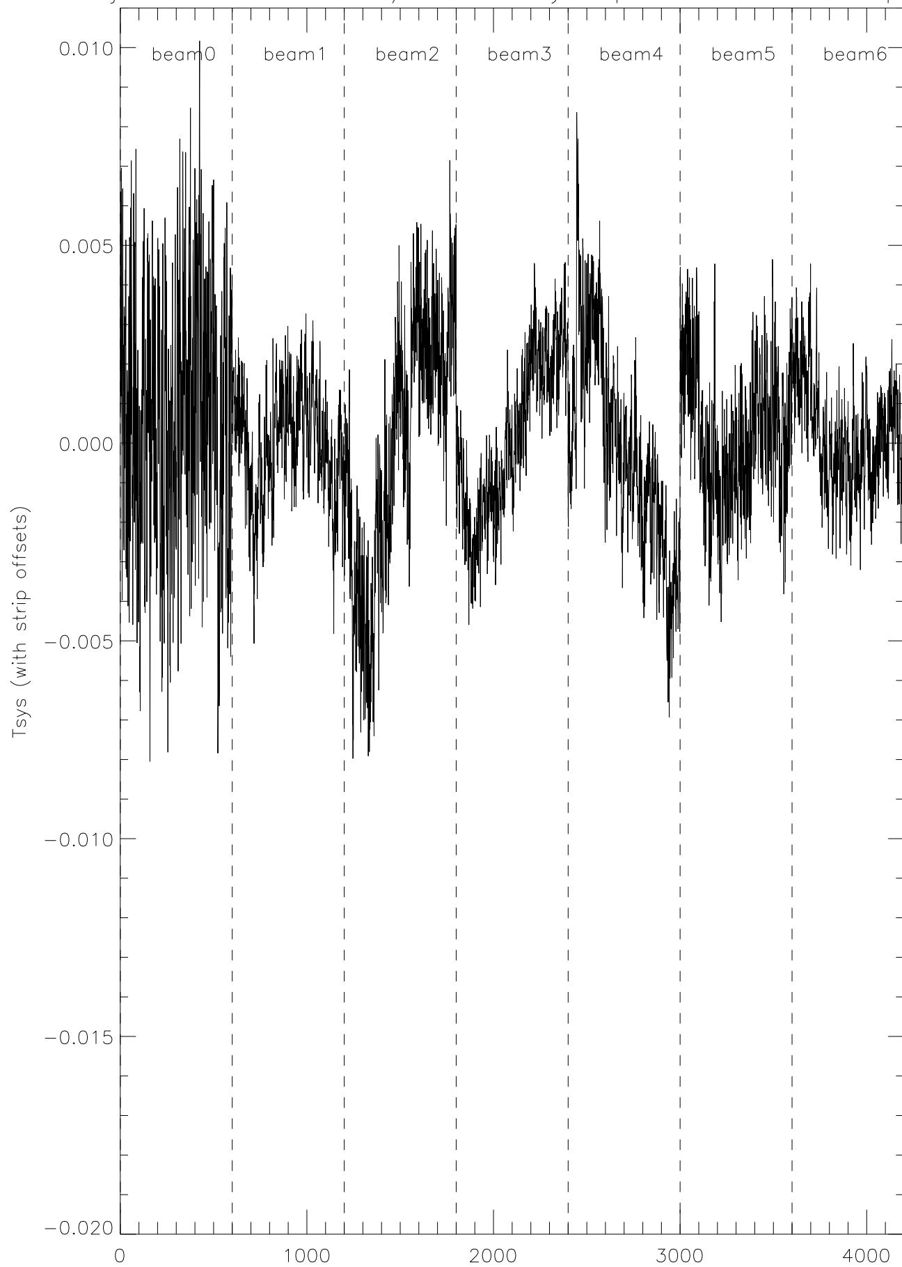
jan08 A2010 TotalPwrA/TotalPwrB by strip and beam.. bad strips
